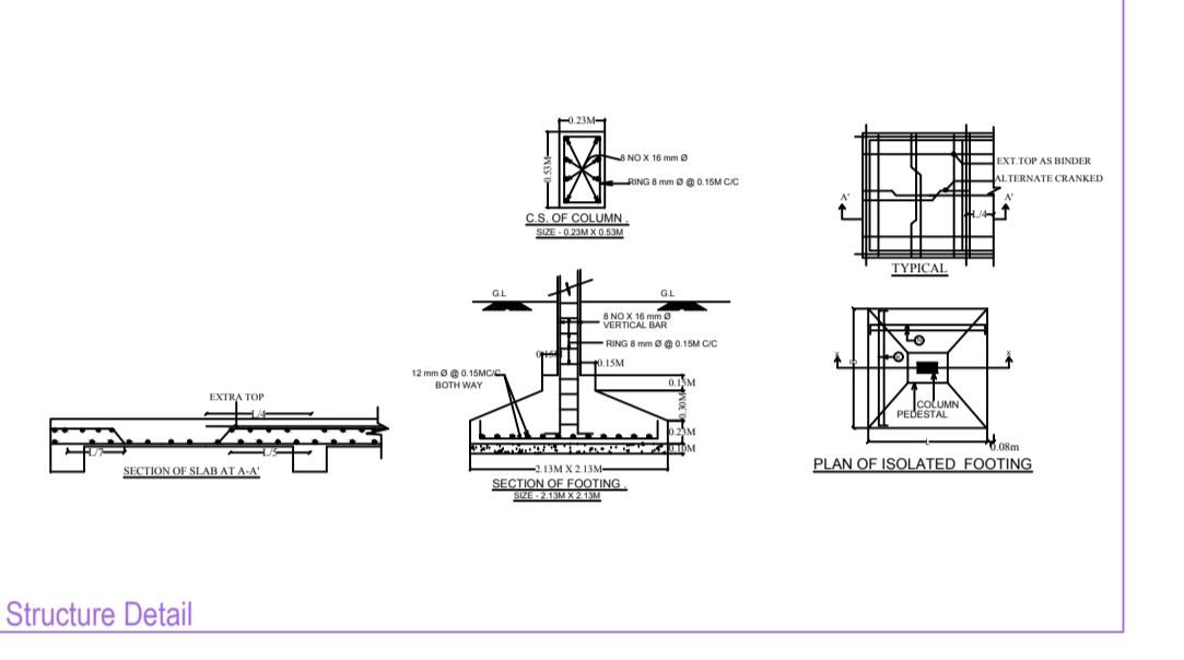
Structure Detail
