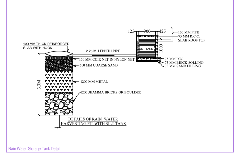
Rain Water Storage Tank Detail
