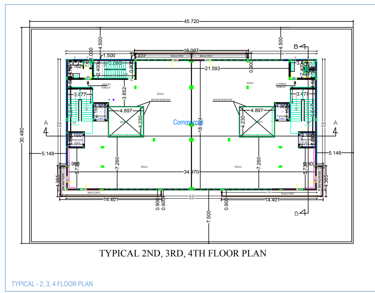
TYPICAL - 2, 3, 4 FLOOR PLAN
