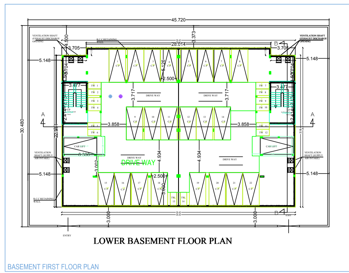
BASEMENT FIRST FLOOR PLAN
