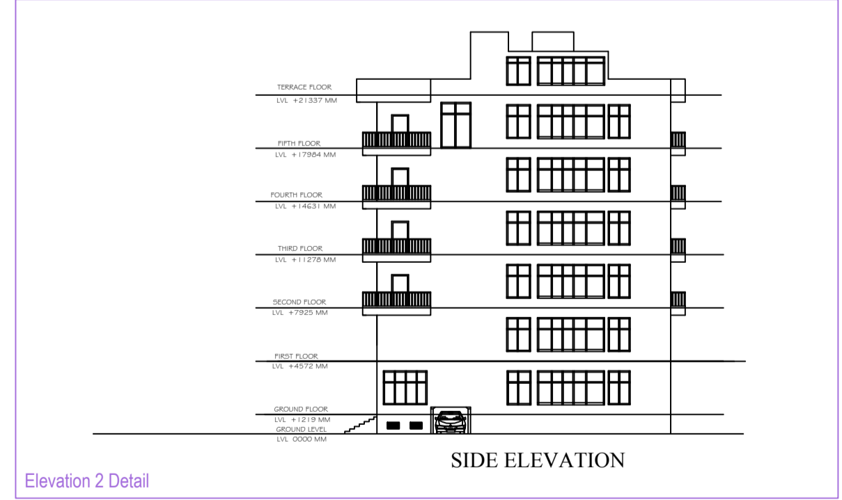
Elevation 2 Detail
