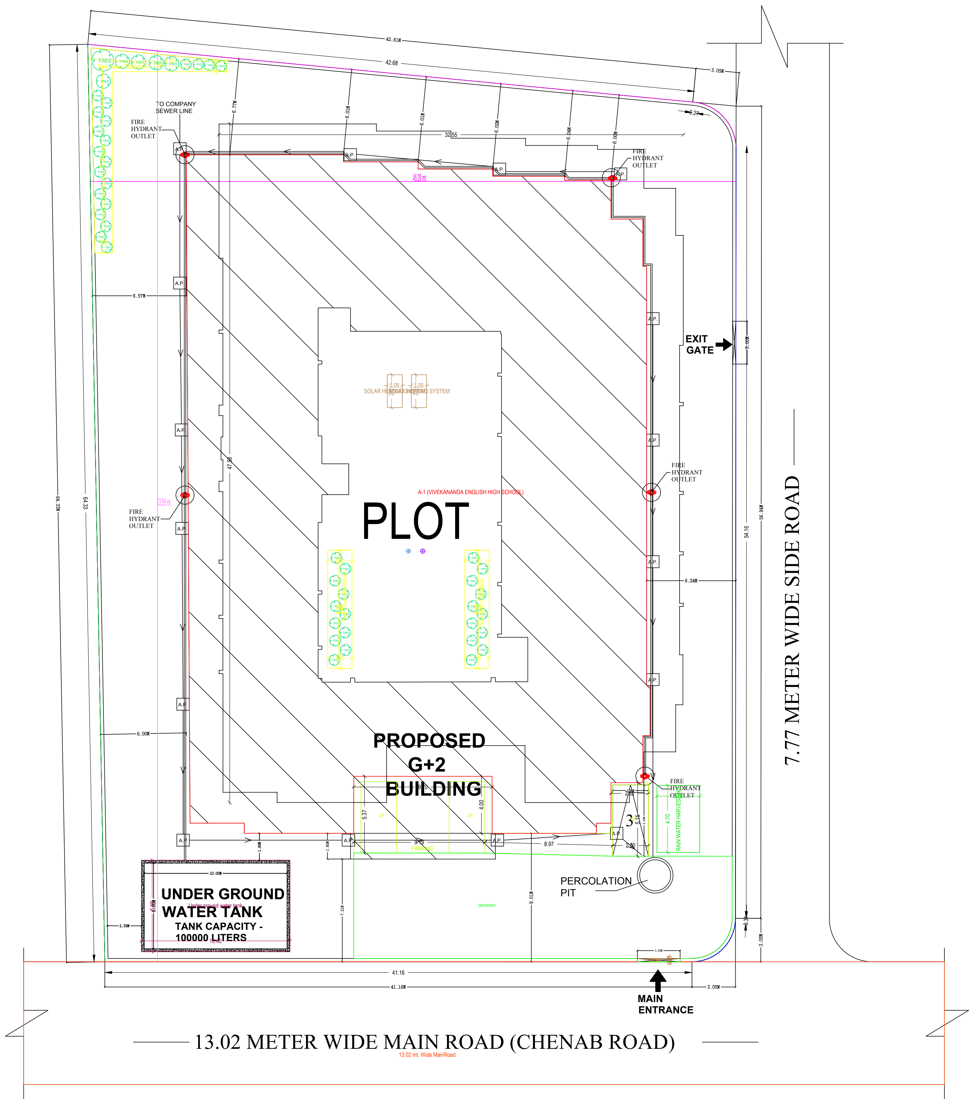
SITE PLAN
