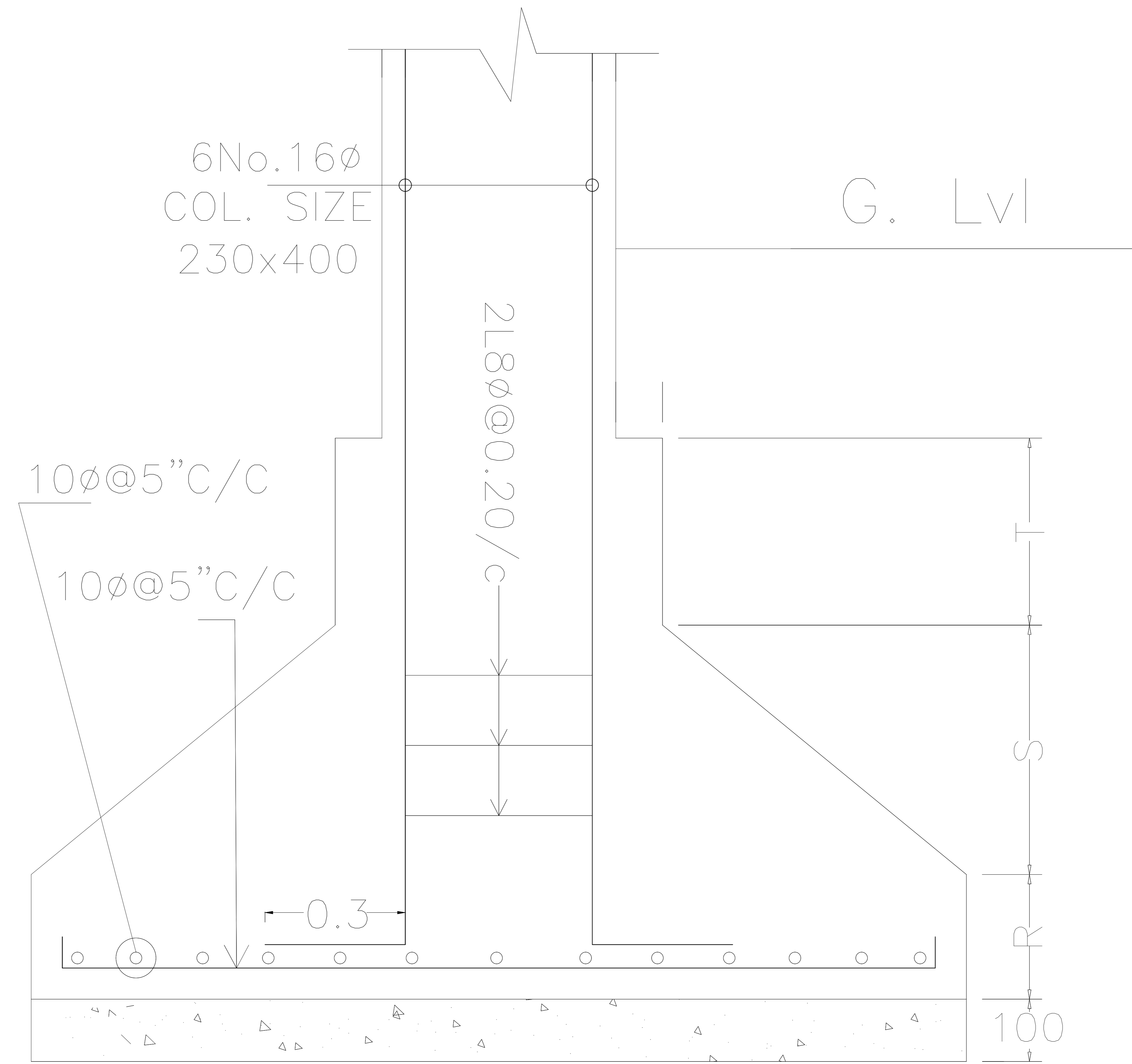
DETAIL OF COLUMN & FOOTING
