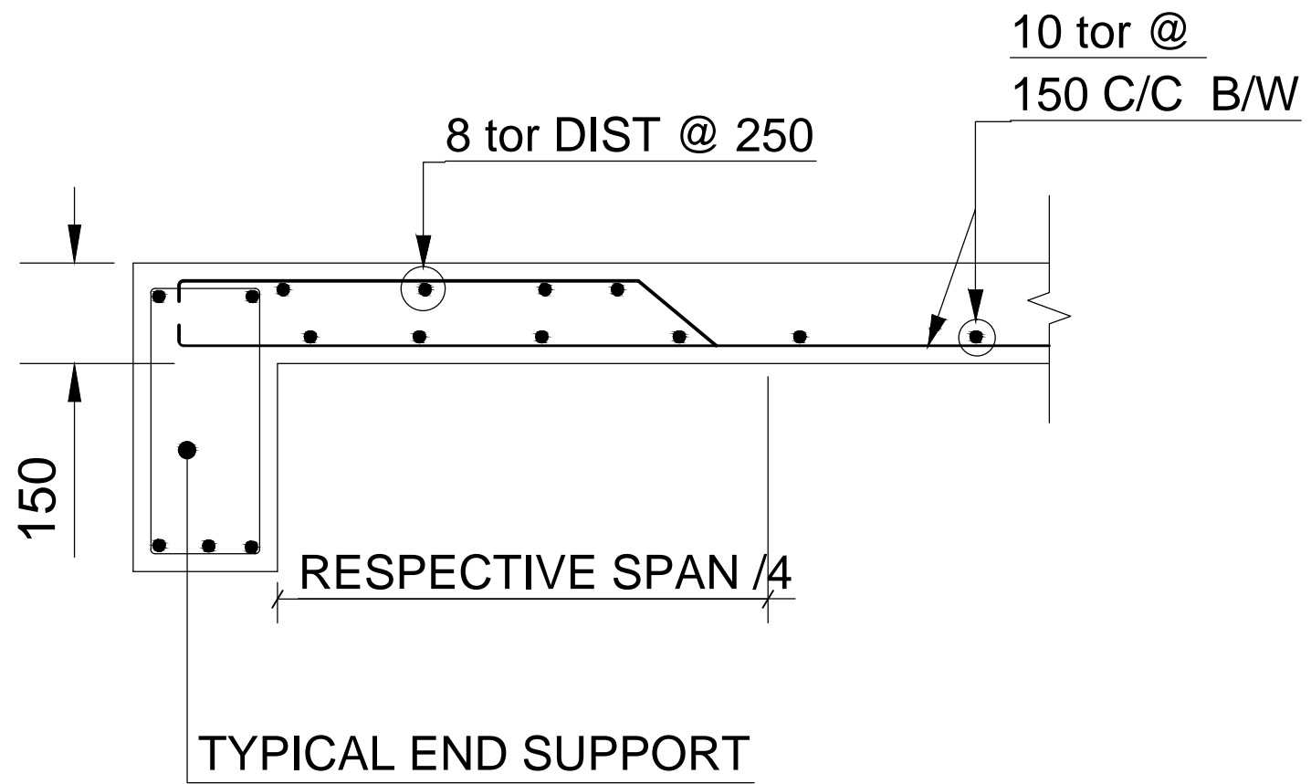
TYPICAL LONG SECTION - FLOOR SLABS
