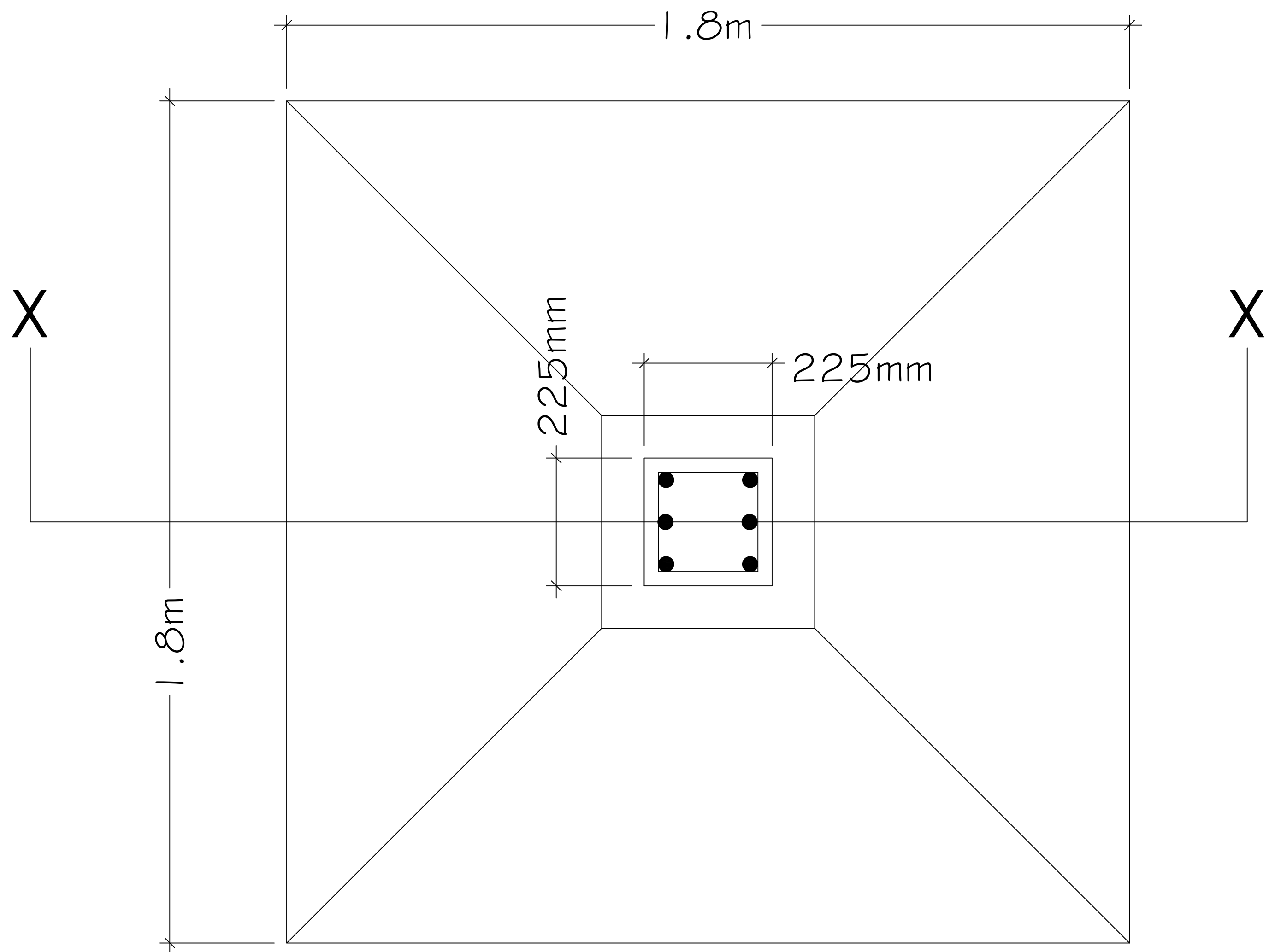
DETAIL OF FOOTING (Not to Scale)
