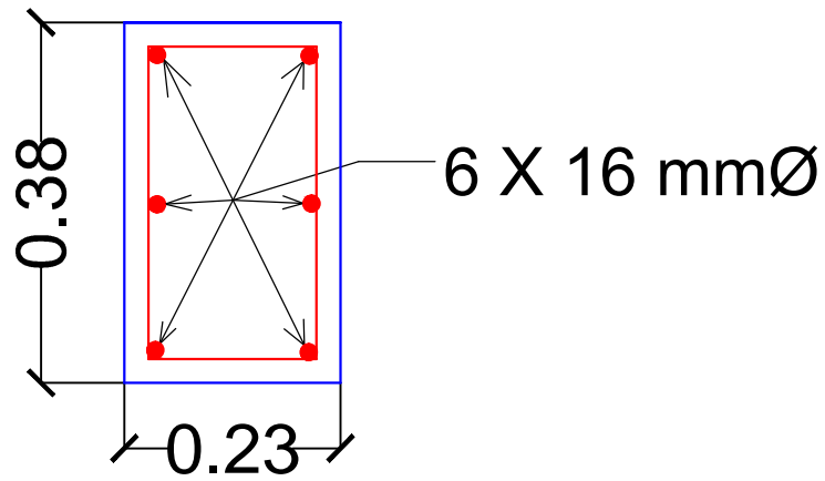
SECTION OF COLUMN.
