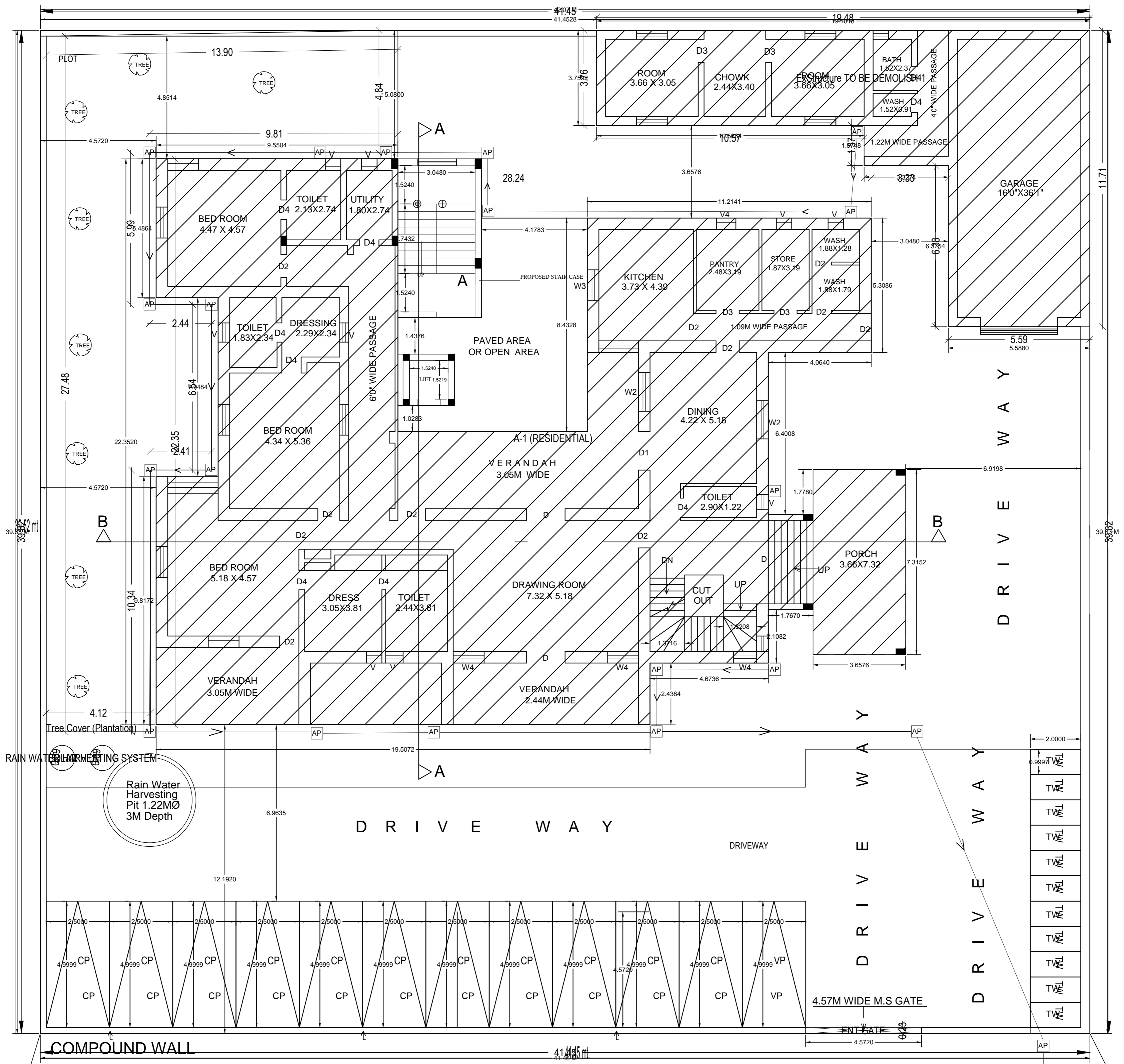
EXISTING GROUND FLOOR PLAN ( WITH SEWER NETWORK ) SCALE 1:100 SOUTH
