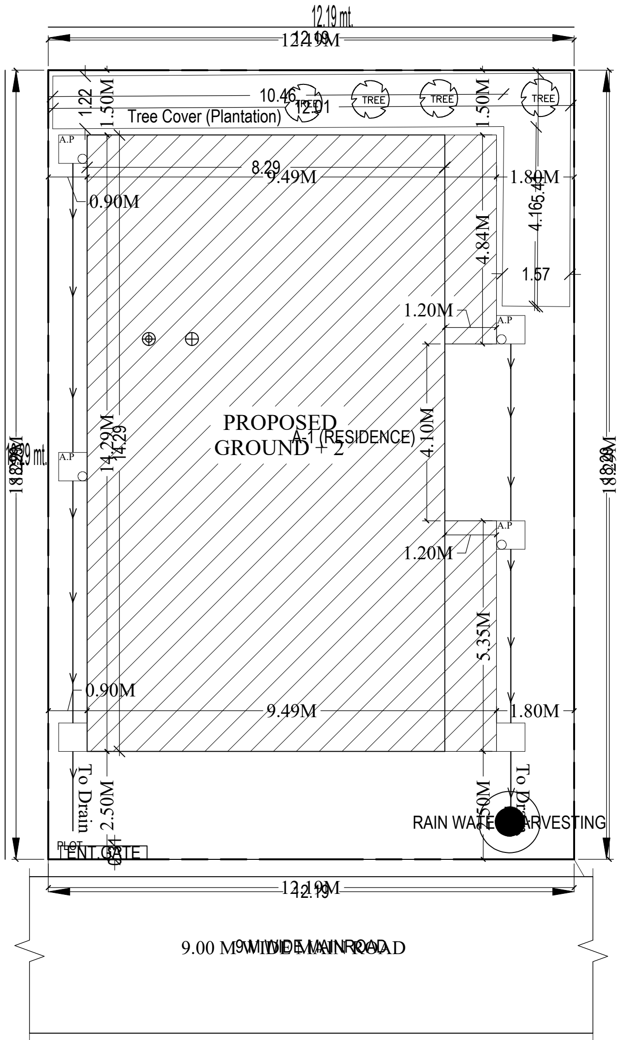
SITE PLAN
