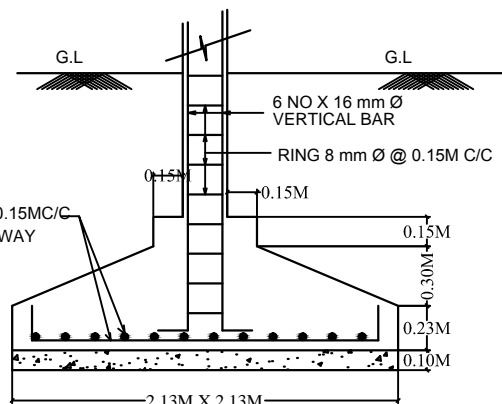
SECTION OF FOOTING . SIZE - 2.13M X 2.13M
