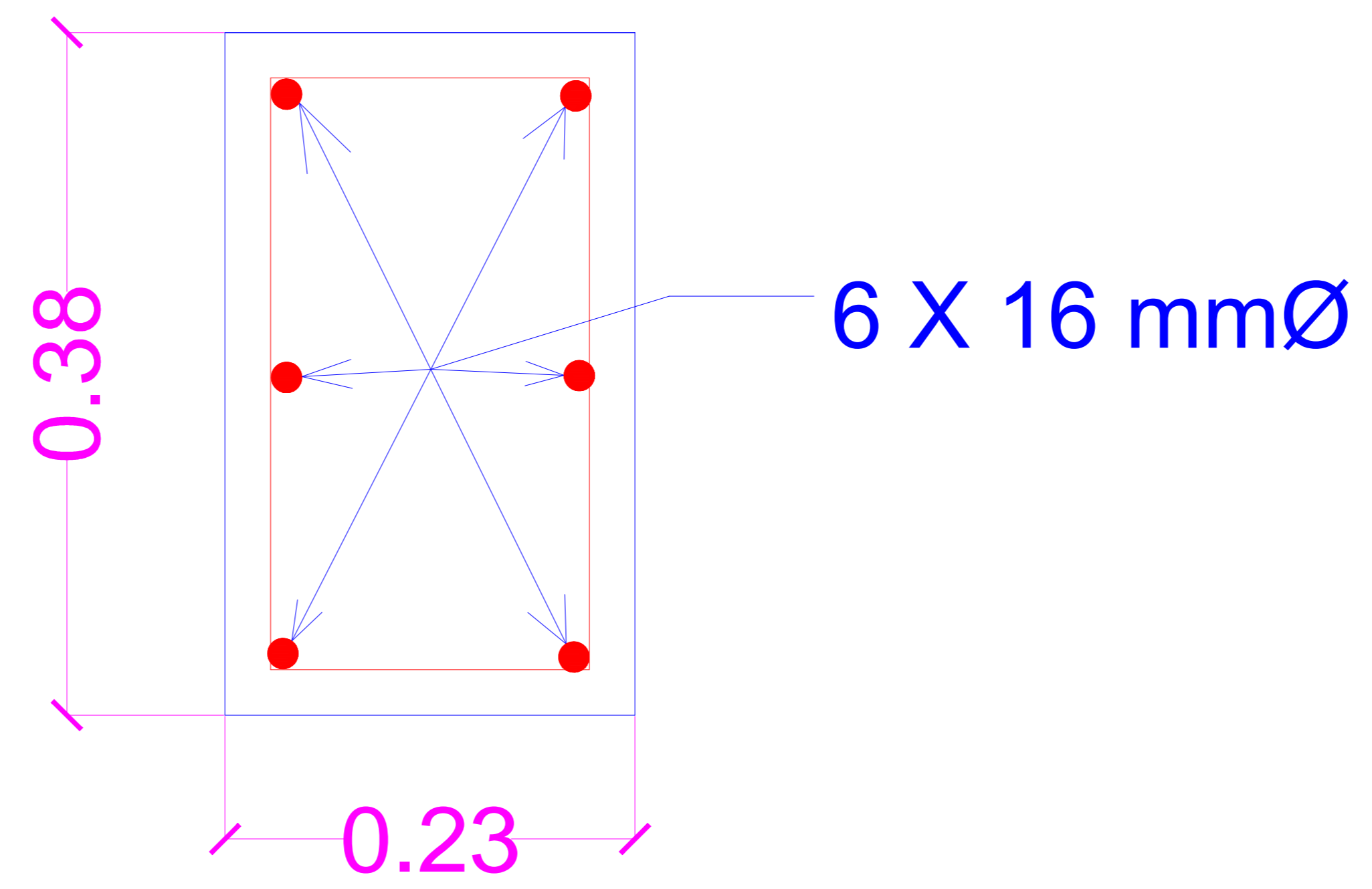
SECTION OF COLUMN.
