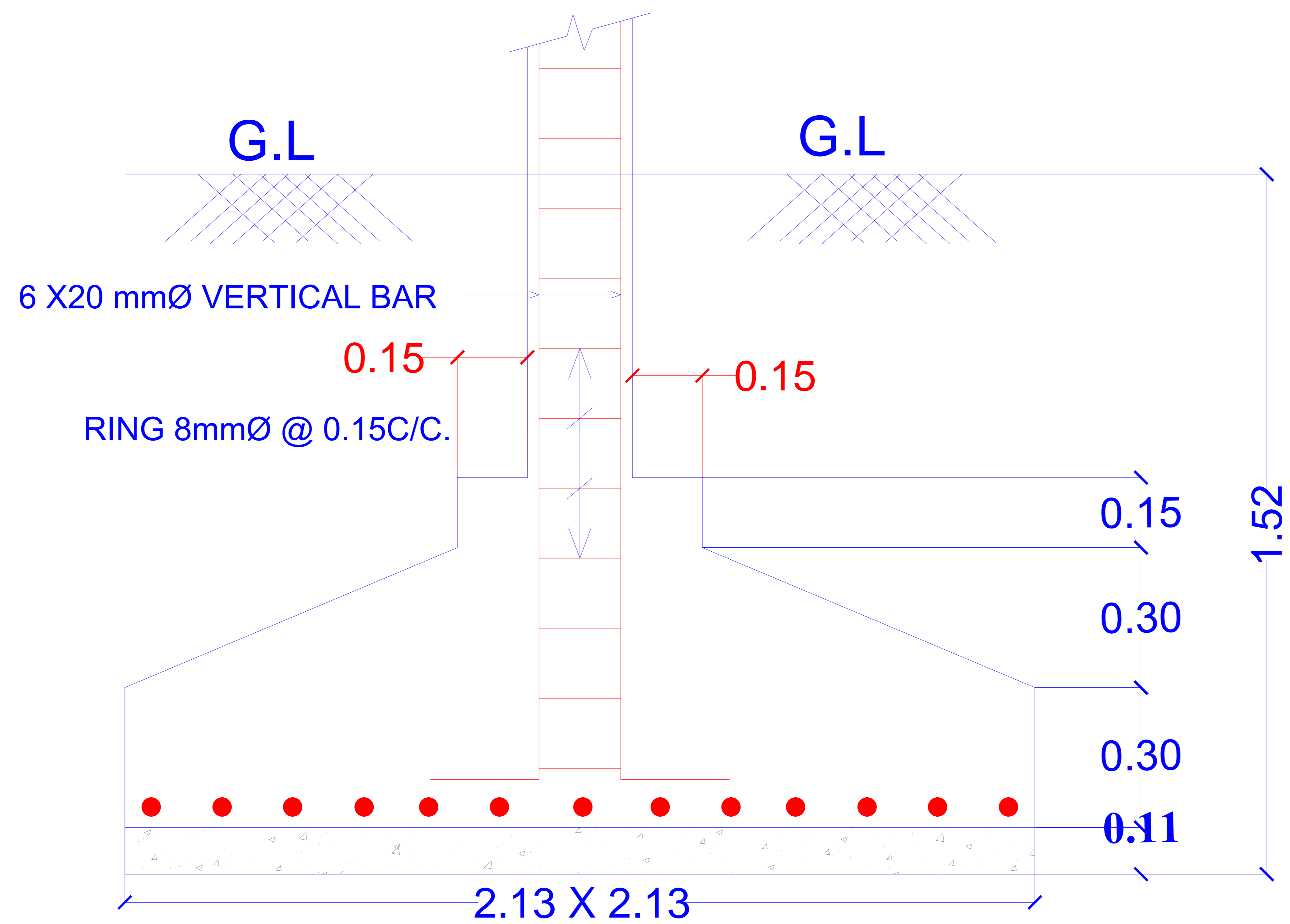
SECTION OF FOOTING
