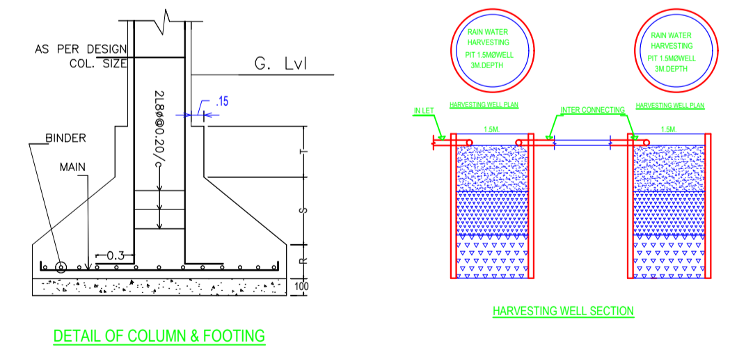
DETAIL OF COLUMN & FOOTING
