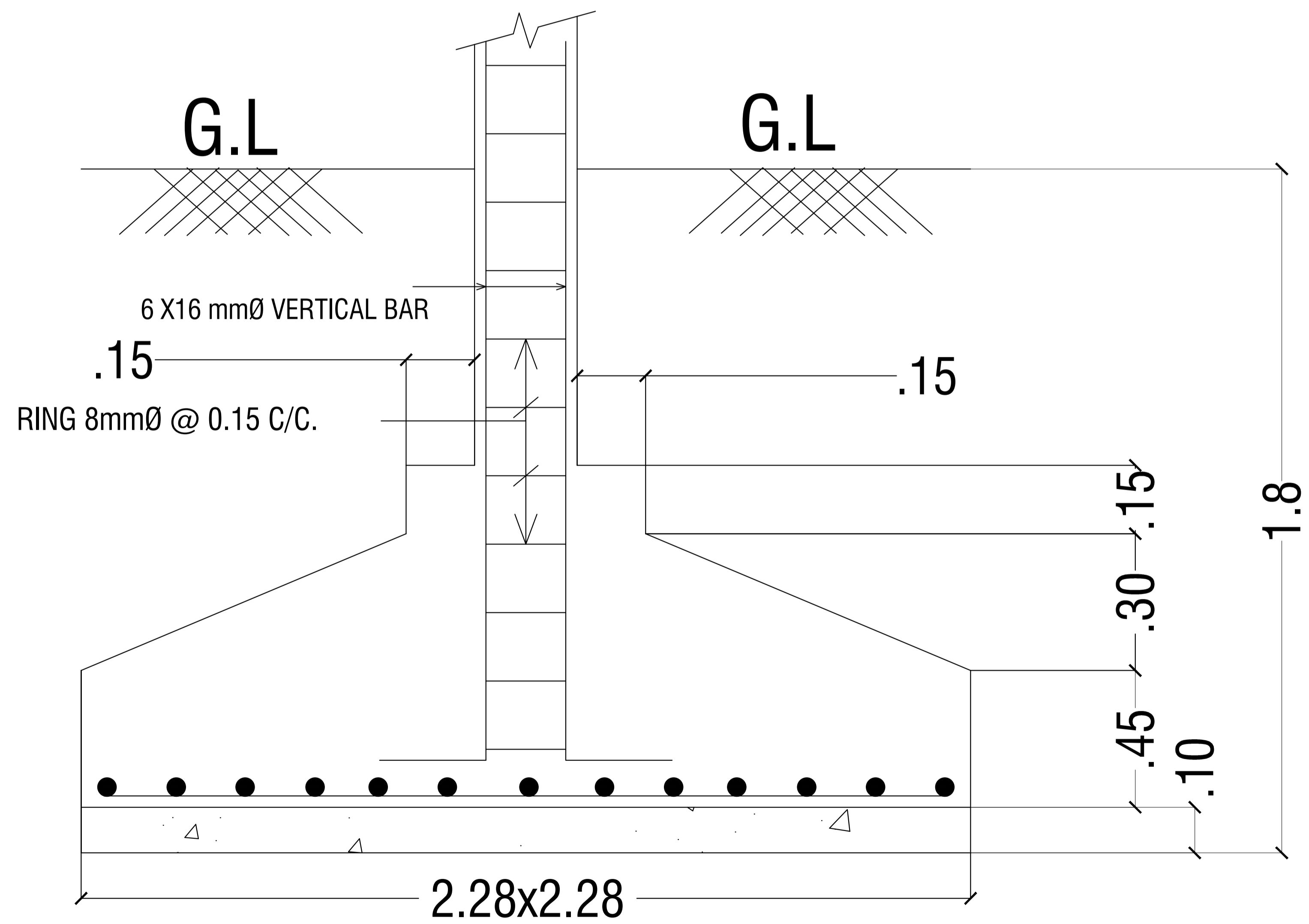
SECTION OF FOOTING
