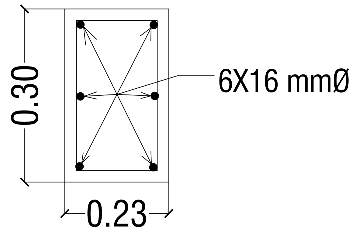
SECTION OF COLUMN
