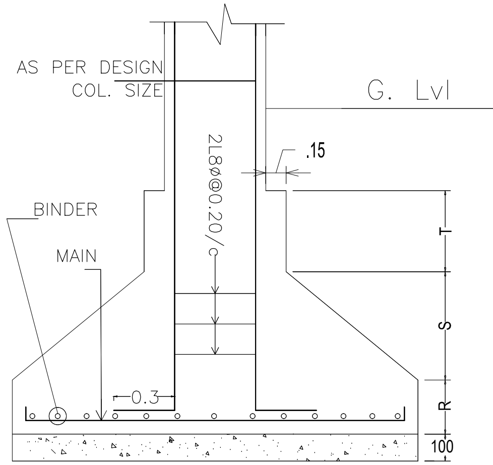
DETAIL OF COLUMN & FOOTING
