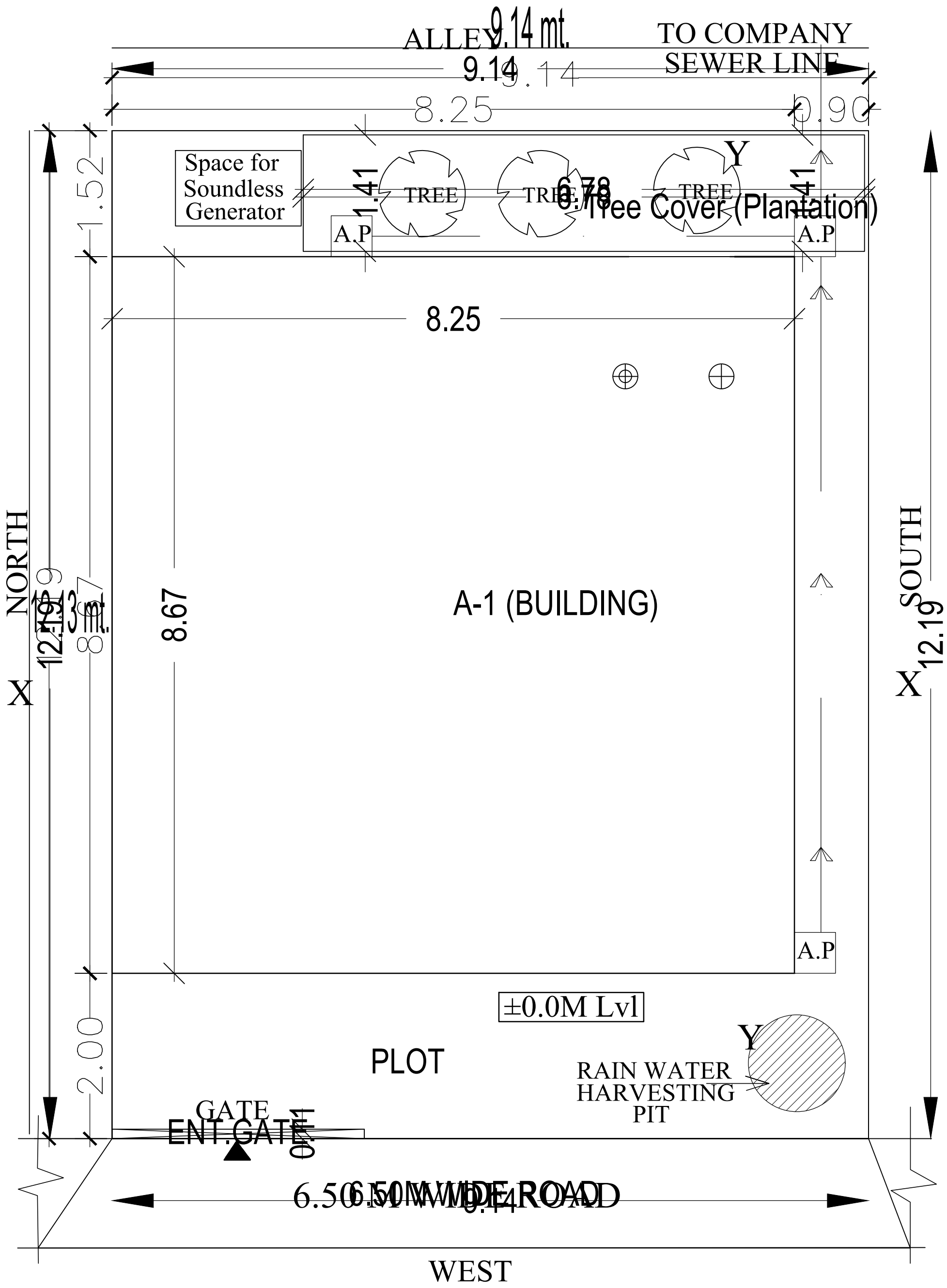
GROUND FLOOR PLAN SHOWING DRAINAGE SCALE-1:100
