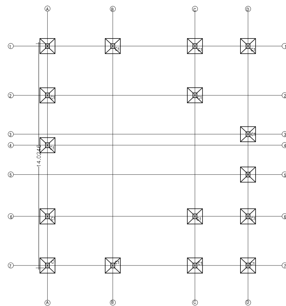
FOOTING PLAN
