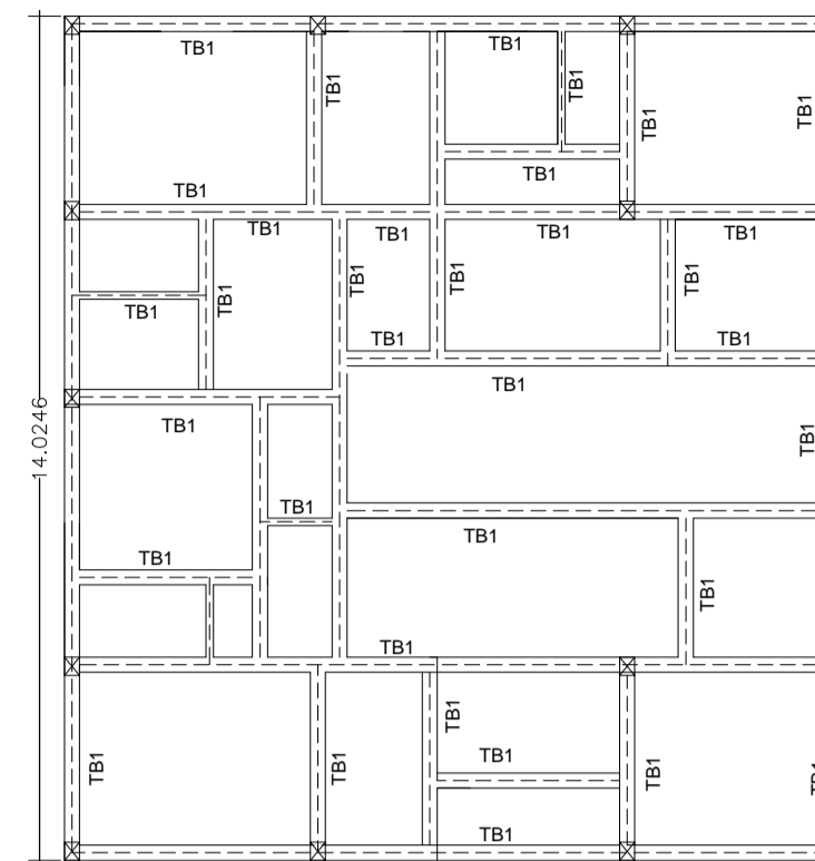
TIE BEAM LAYOUT PLAN
