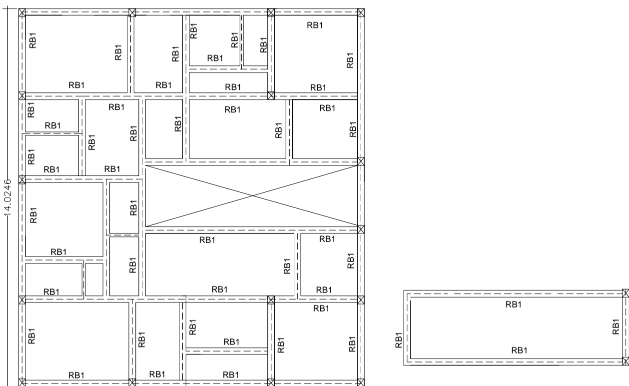
MUMTY ROOF BEAM LAYOUT PLAN
