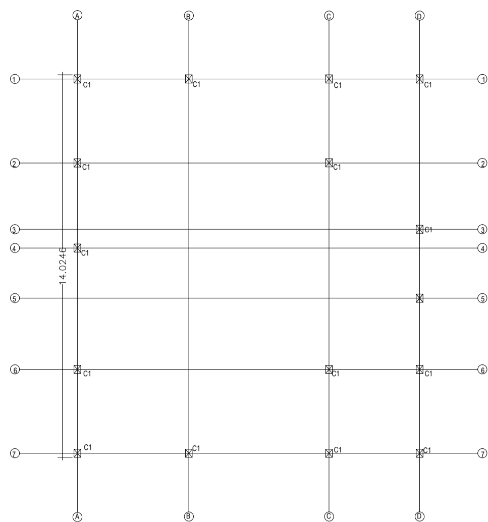
COLUMN CENTER LINE PLAN
