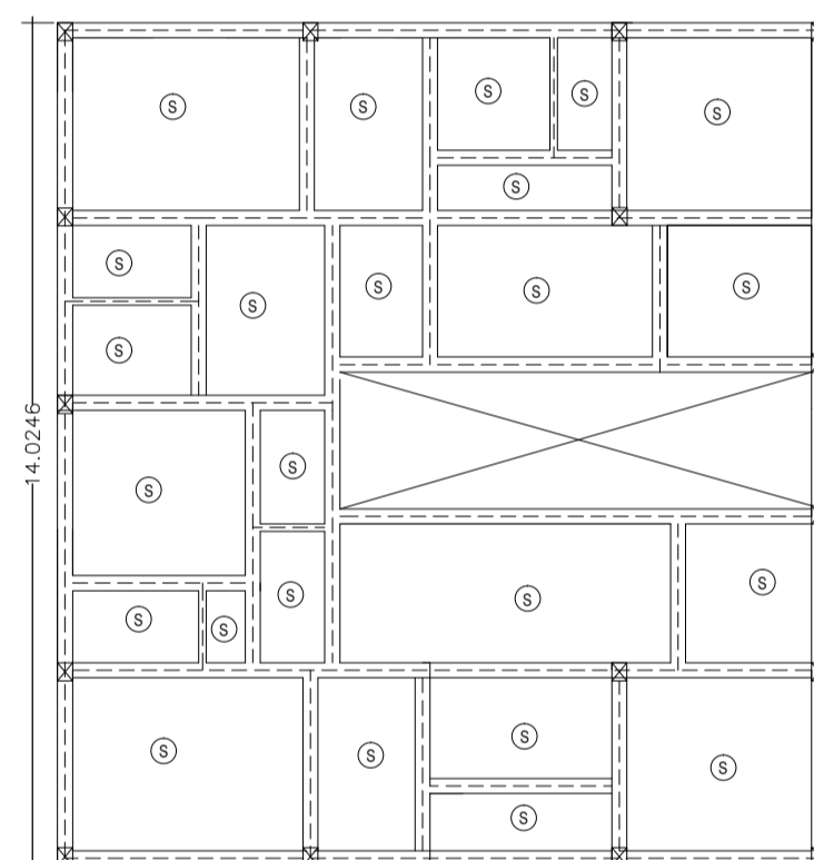
TYPICAL ROOF SLAB LAYOUT PLAN
