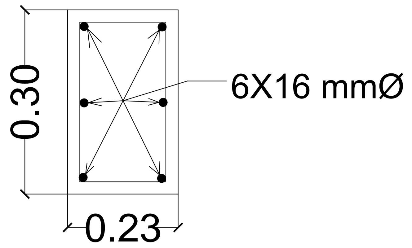
SECTION OF COLUMN
