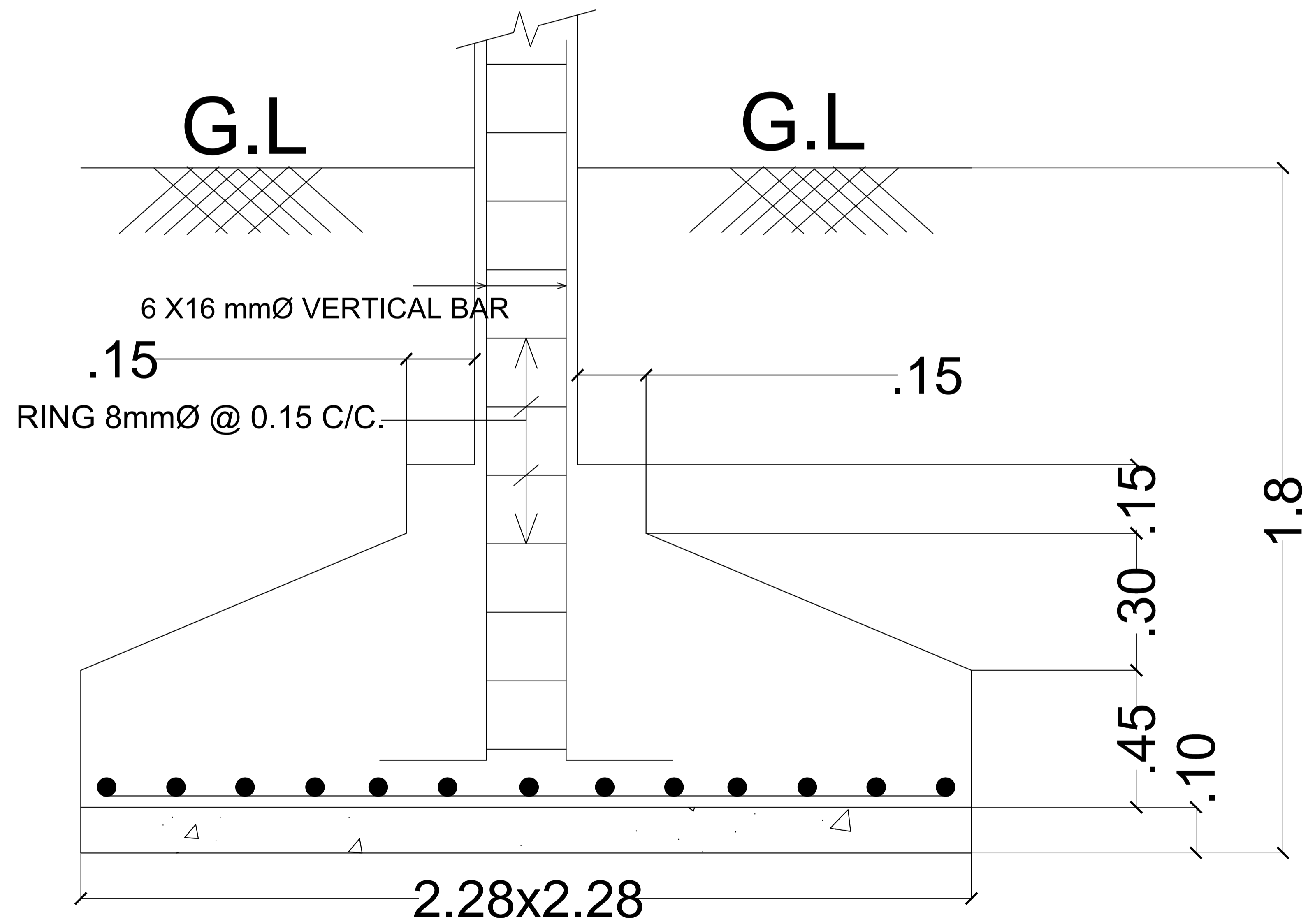
SECTION OF FOOTING
