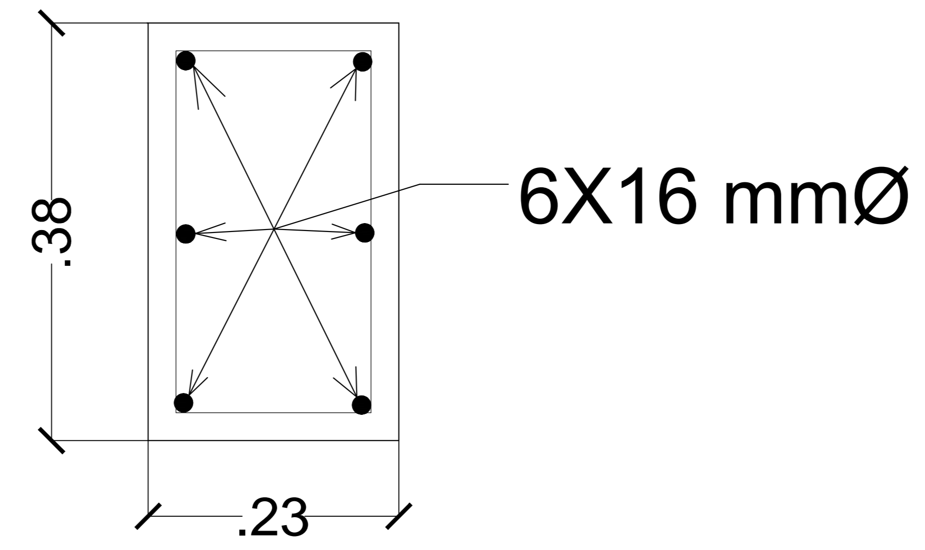
SECTION OF COLUMN. - C1
