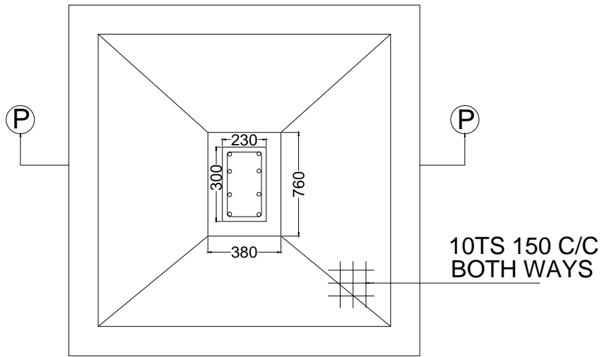
PLAN FOOTING PLAN (AS/STRL. DESIGN) SCALE N.T.S
