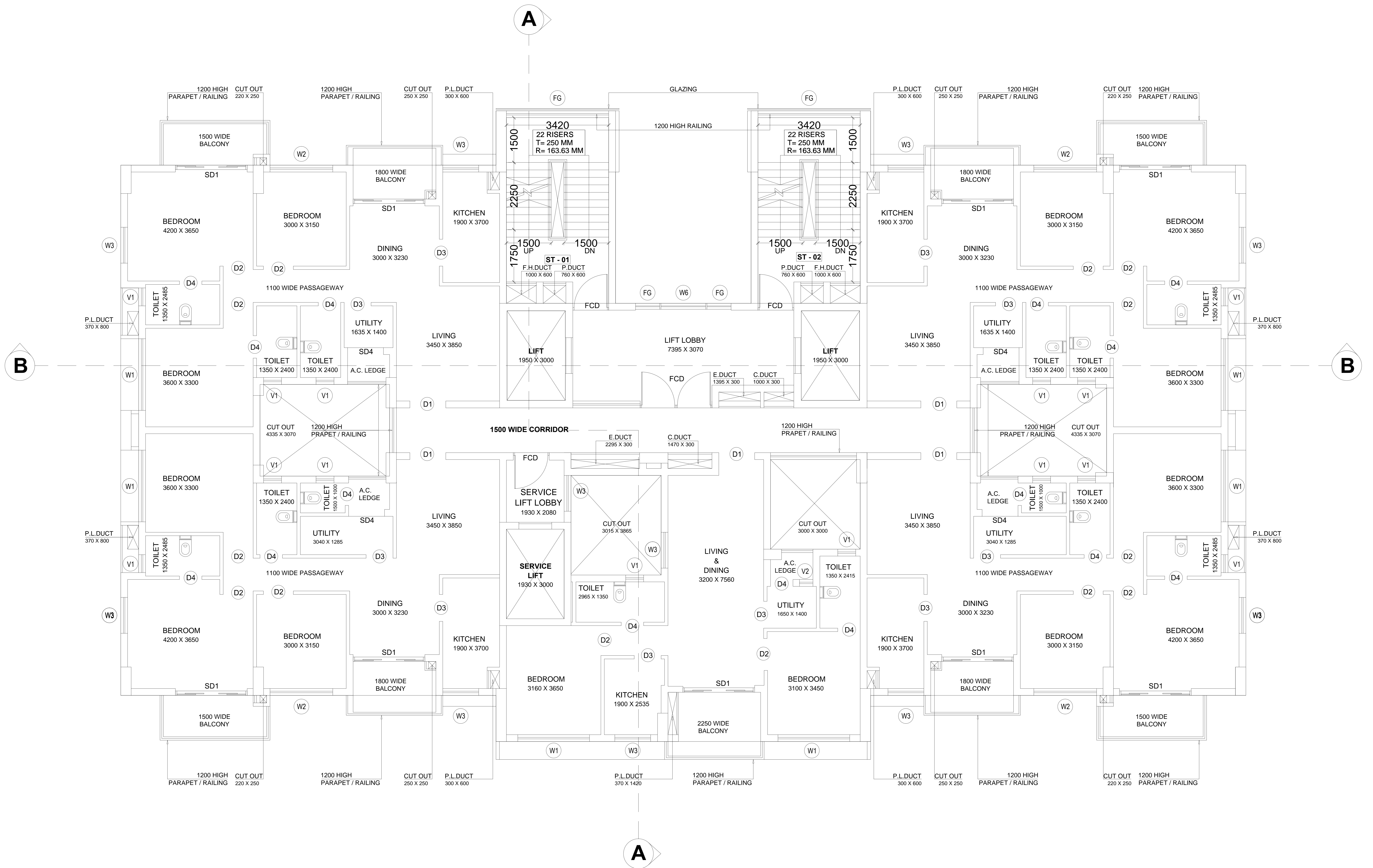
TYPICAL PLAN ( 4TH FLOOR )
