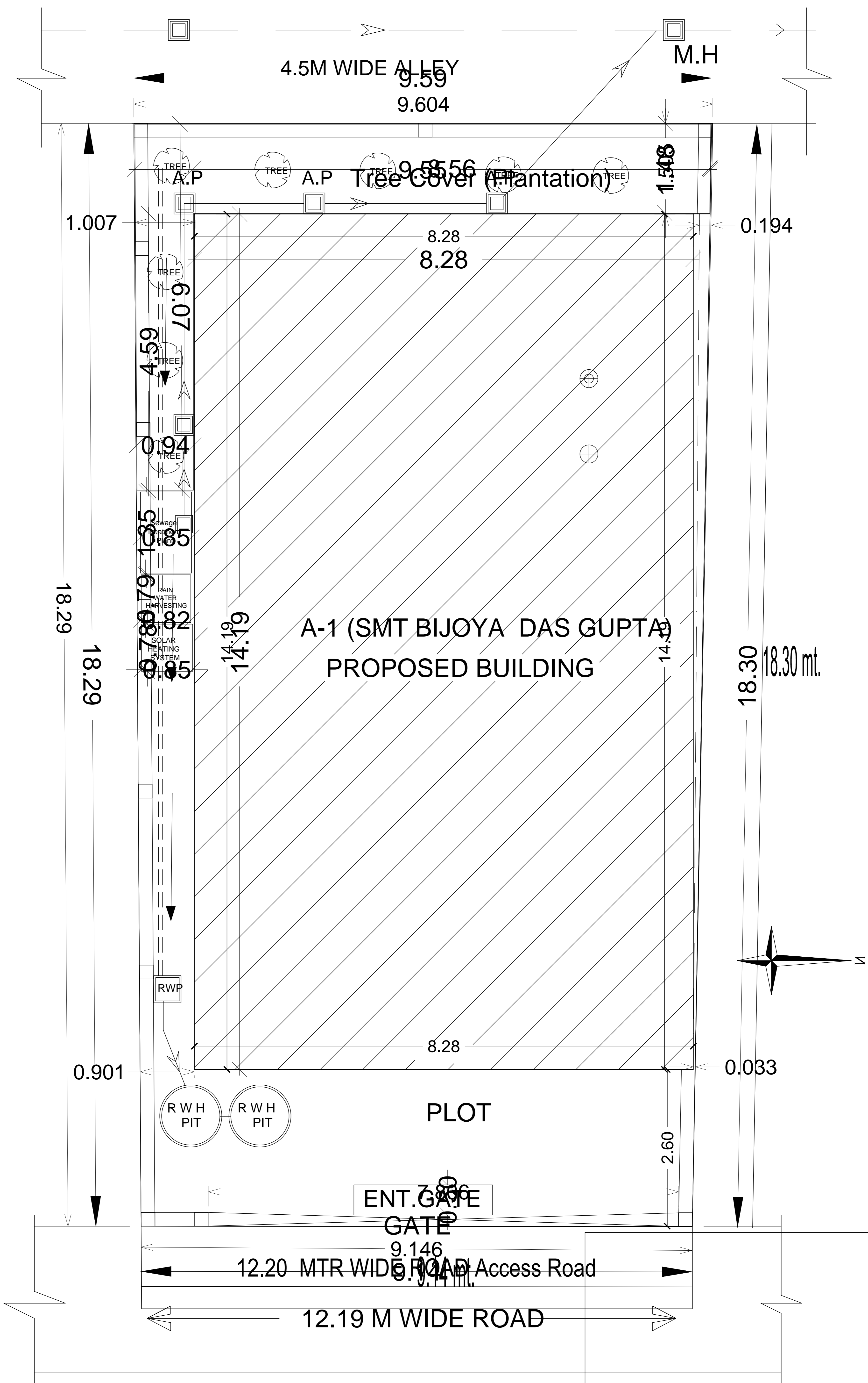
SITE PLAN (SCALE=1:100)
