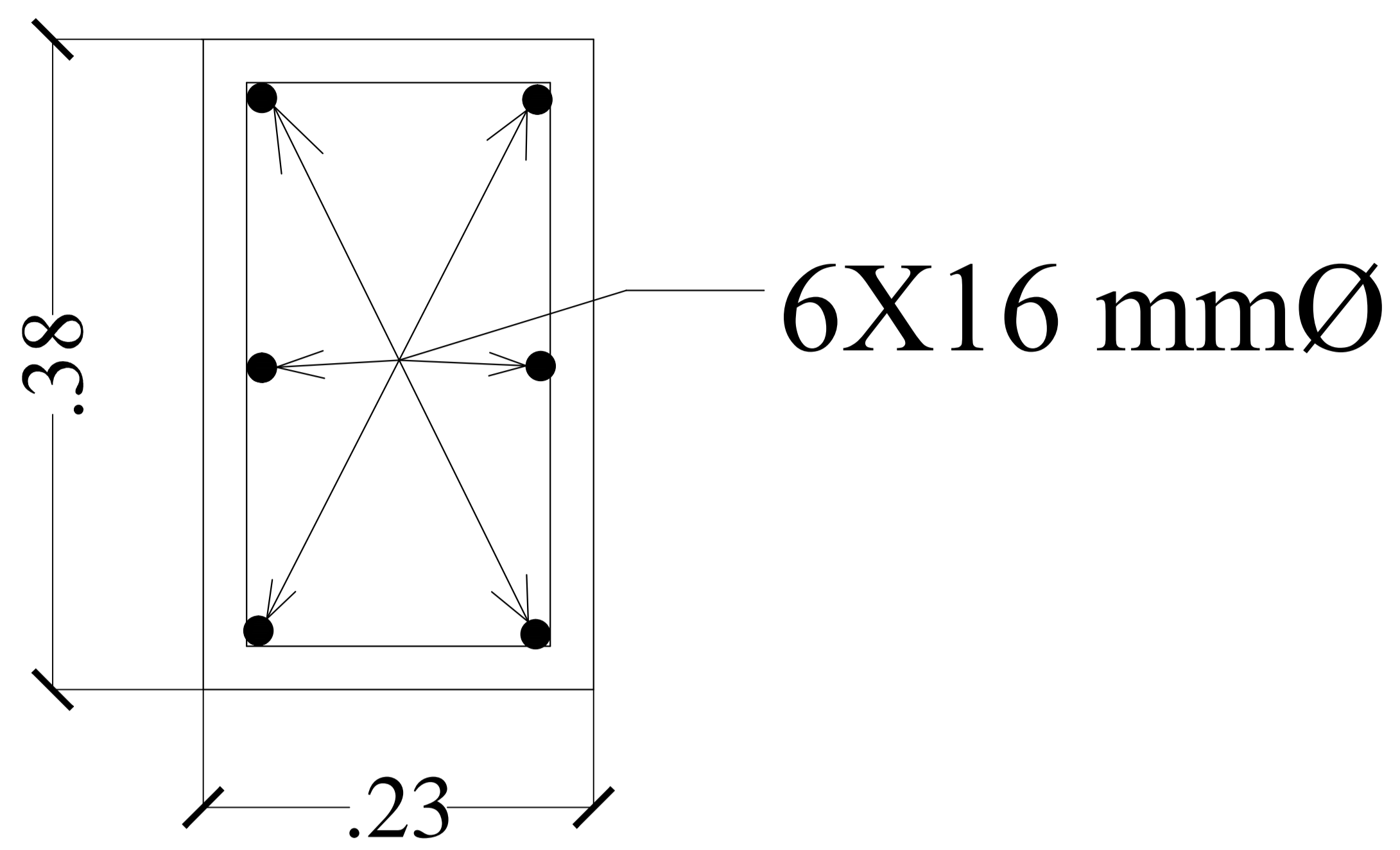
SECTION OF COLUMN. - C1
