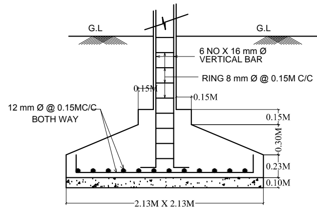
SECTION OF FOOTING . SIZE - 2.13M X 2.13M
