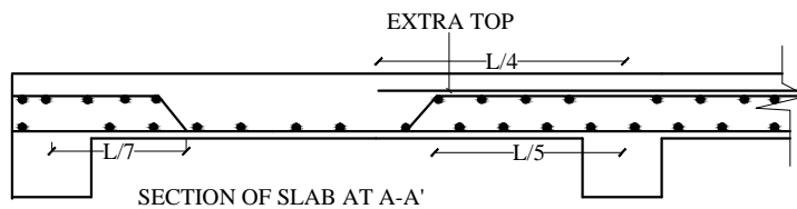
SECTION OF SLAB AT A-A'
