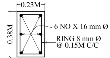
C.S. OF COLUMN . SIZE - 0.23M X 0.38M
