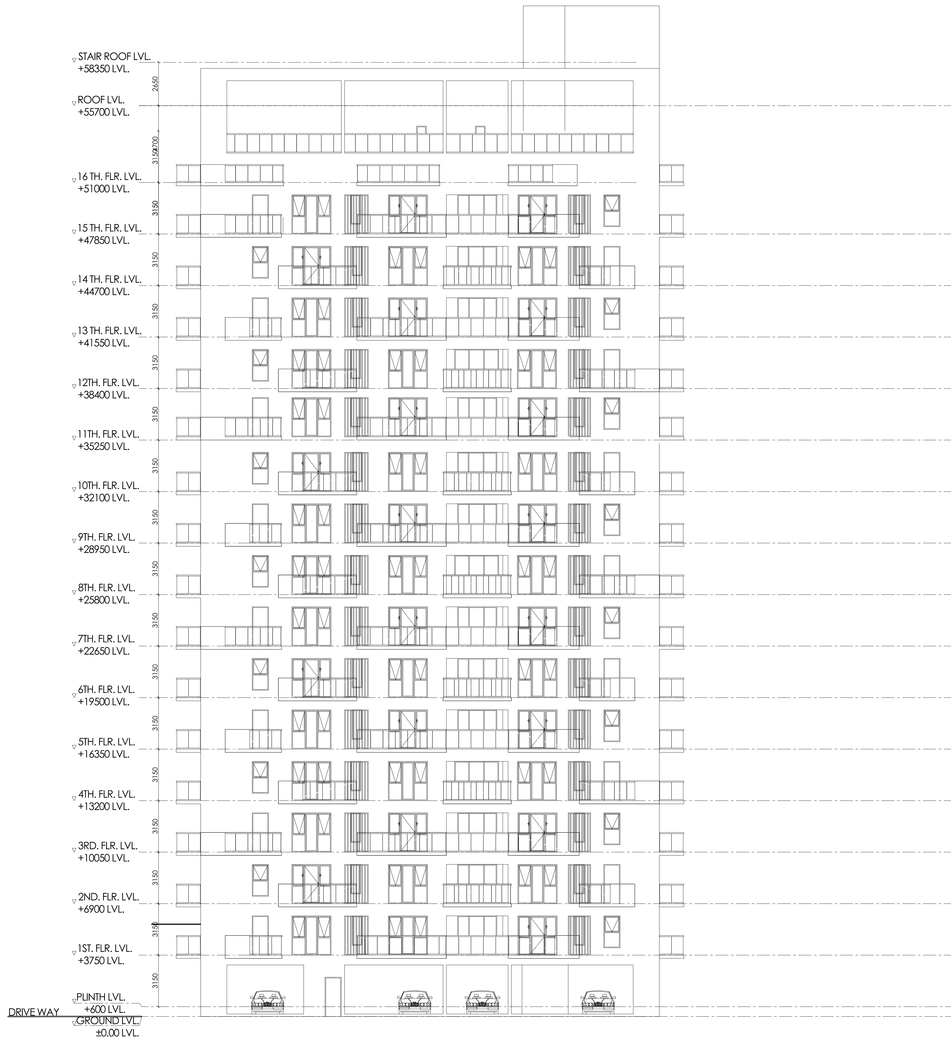
RIGHT SIDE ELEVATION
