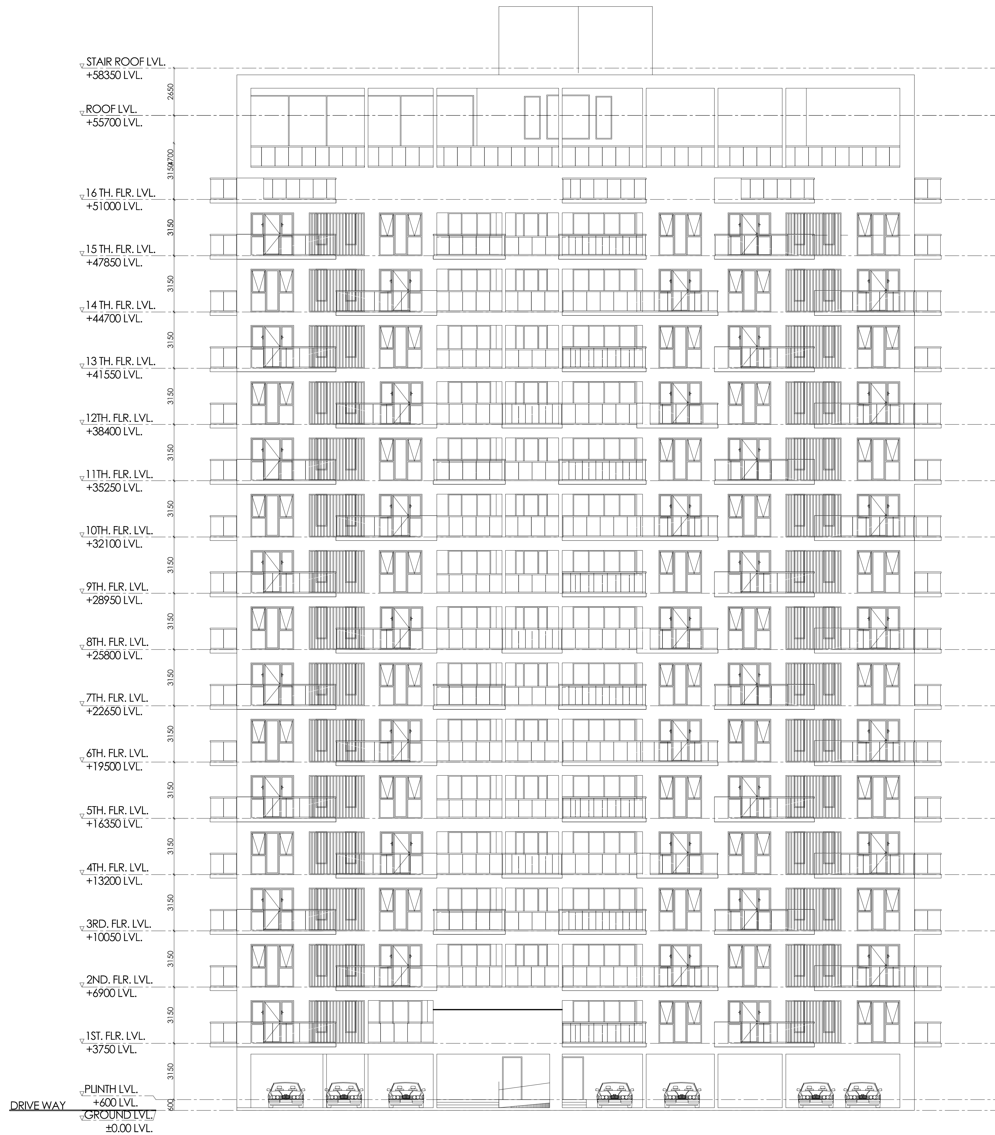
FRONT ELEVATION
