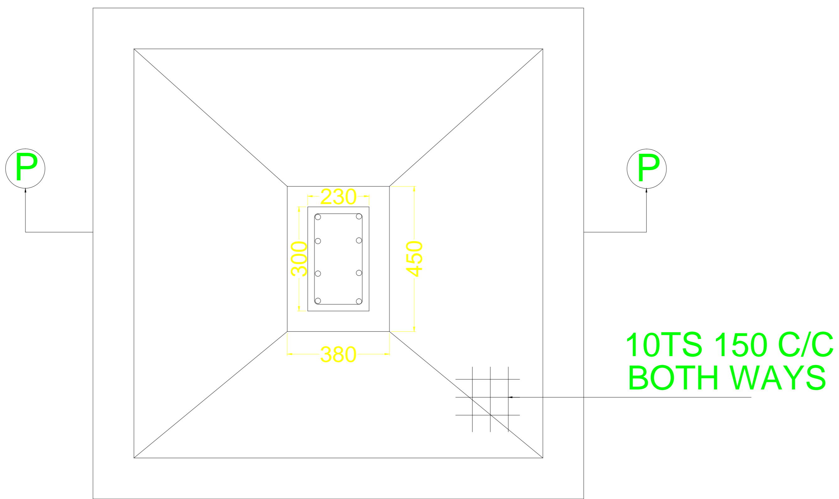
PLAN FOOTING PLAN (AS/STRL. DESIGN) SCALE N.T.S
