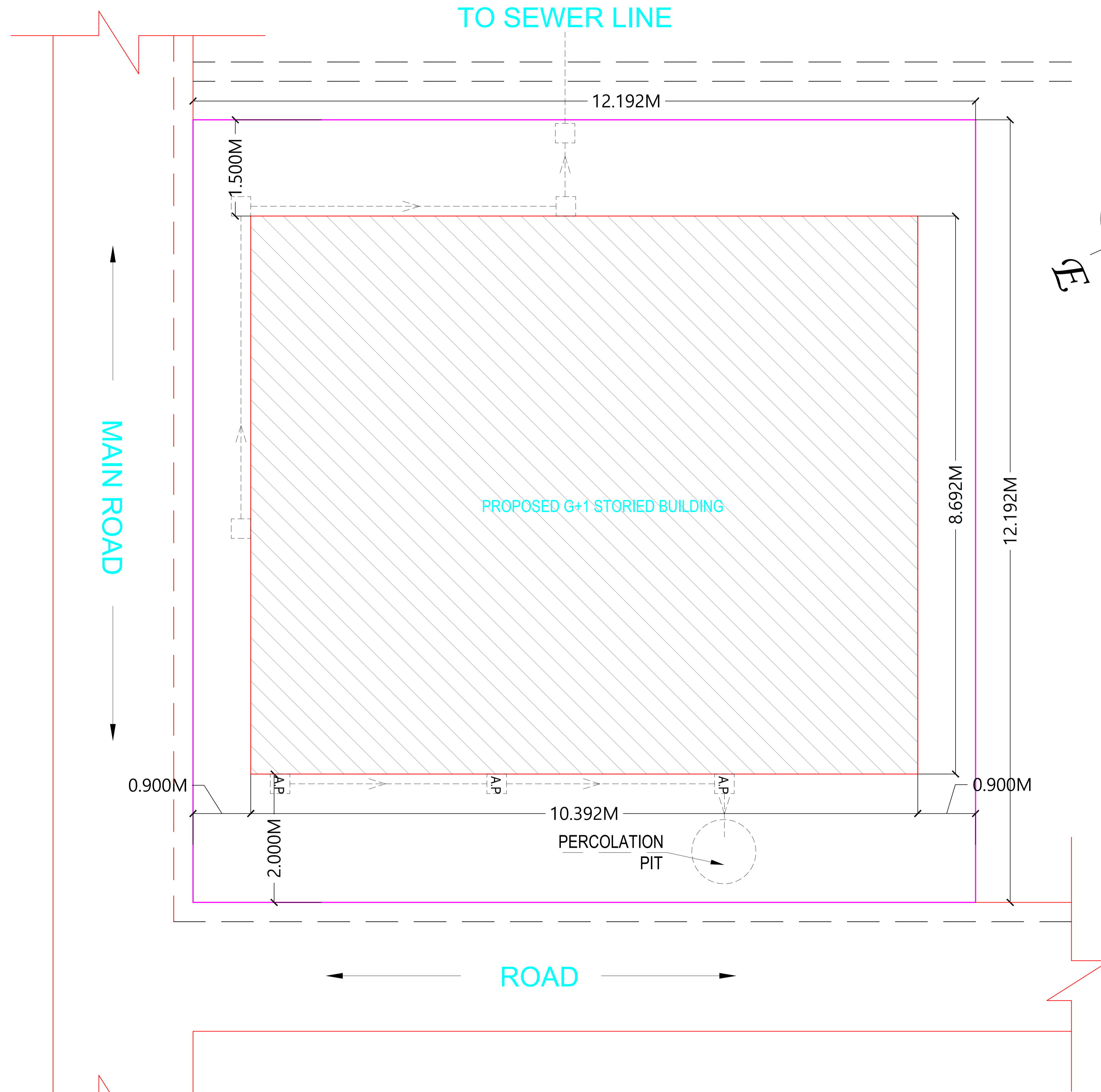
SITE PLAN
