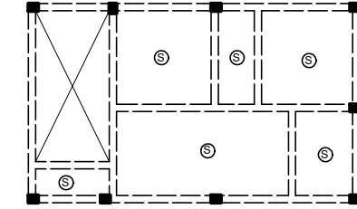
GROUND & FIRST SLAB LAYOUT PLAN
