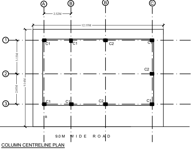
COLUMN CENTRELINE PLAN
