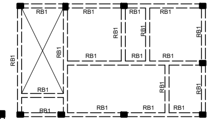
GROUND & FIRST ROOF BEAM LAYOUT PLAN
