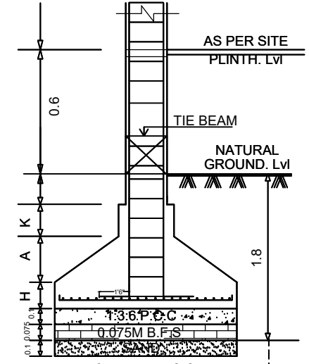
TYPICAL DETAILS OF SECTIONAL ELEVATION
