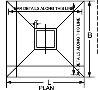
TYPICAL DETAILS OF COLUMN FOOTING
