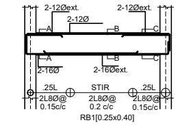
GROUND & FIRST ROOF BEAM LAYOUT PLAN
