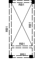
MUMTY ROOF BEAM LAYOUT PLAN
