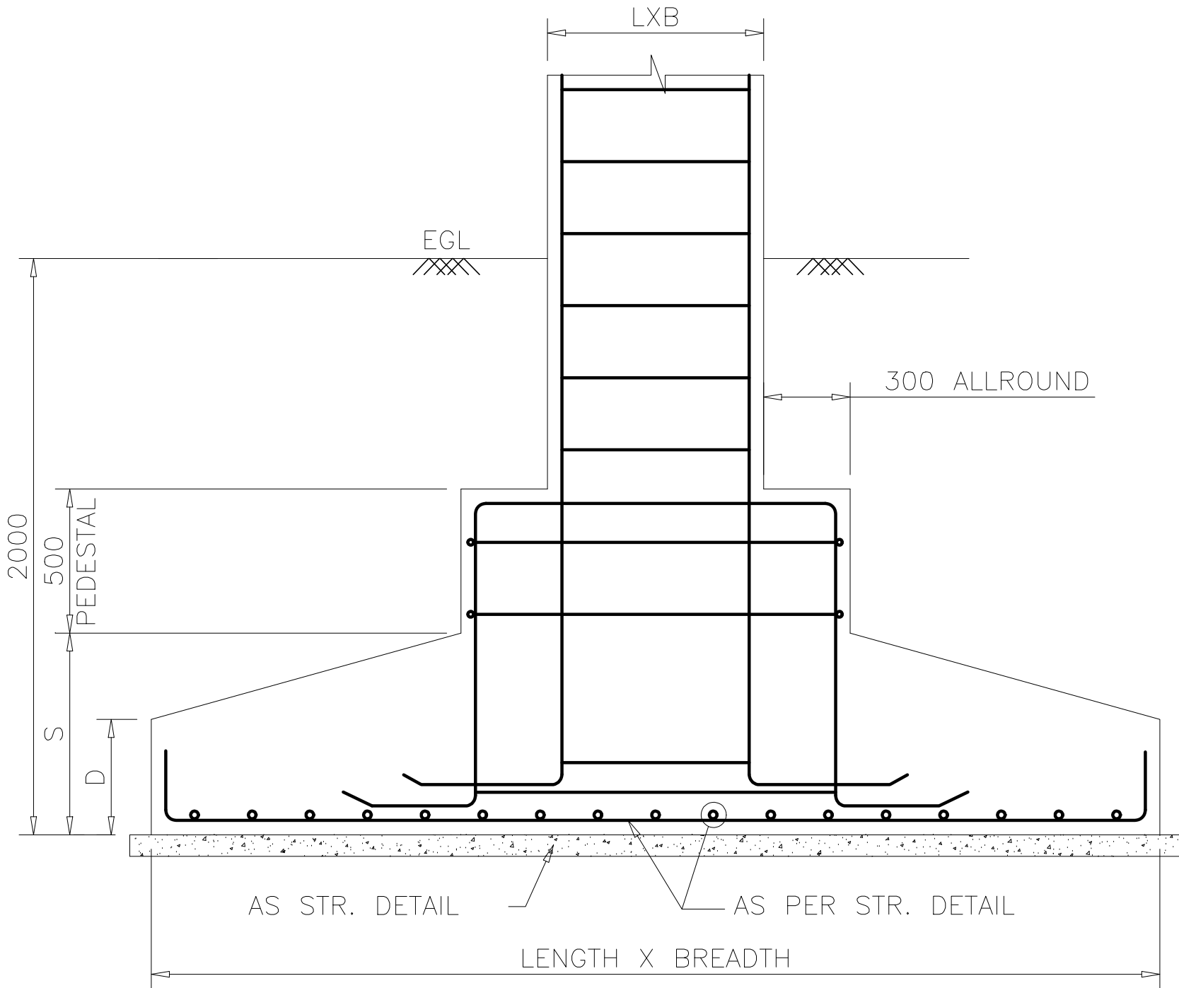
TYPICAL FOOTING DETAILS
