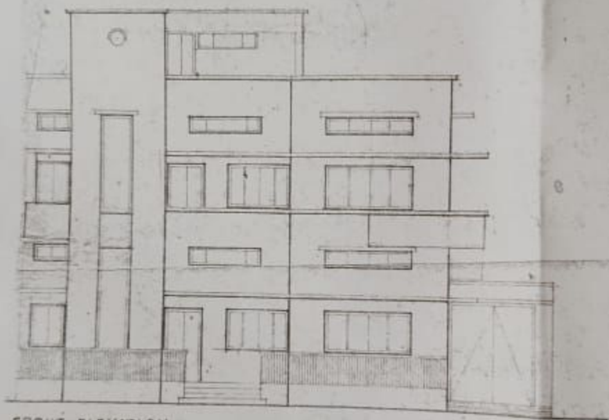
FRONT ELEVATION (SCALE: 1" = 8 FT.)
