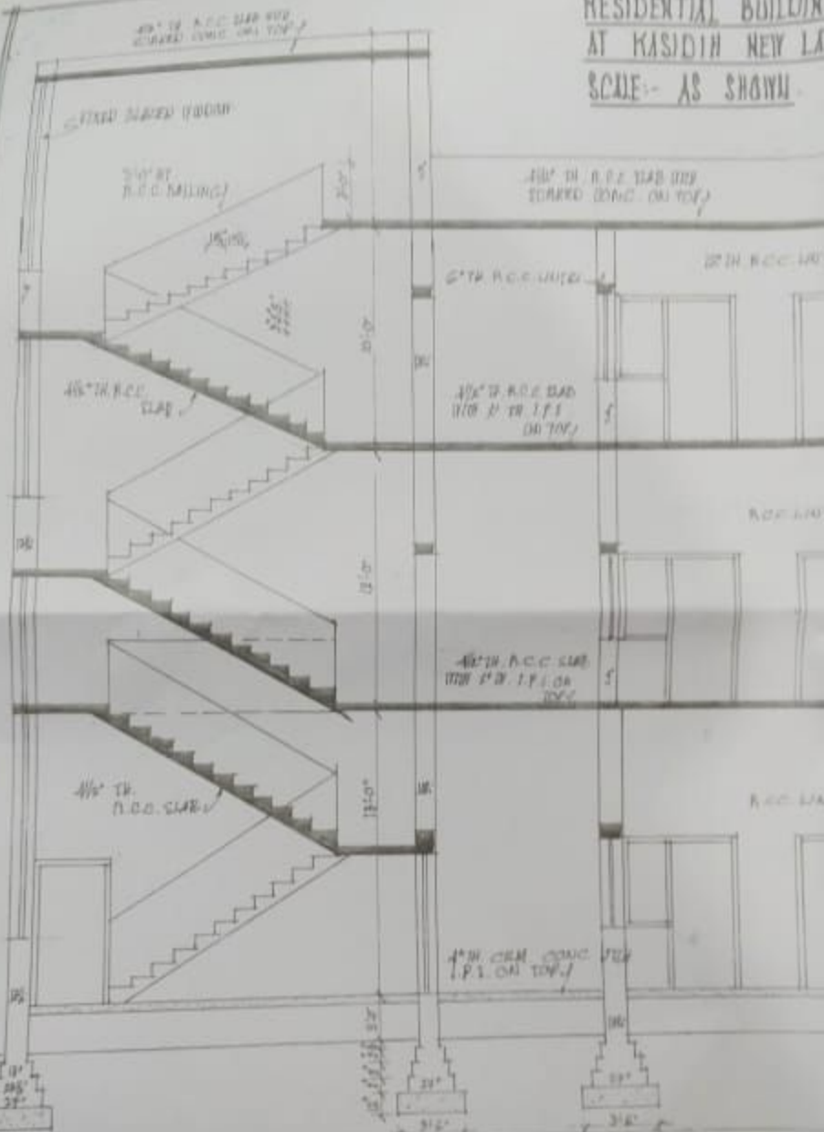
SECTION AT A-A, SCALE:- 1" = 4'-0"
