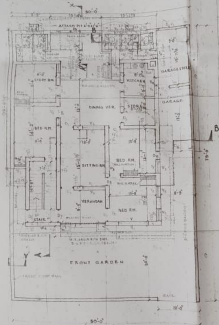
GROUND FLOOR PLAN scale: 1"=8ft
