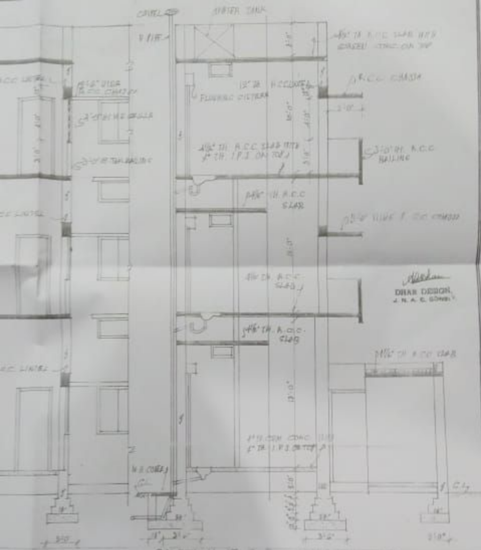
SECTION AT B-B, SCALE: 1" = 4'-0"
