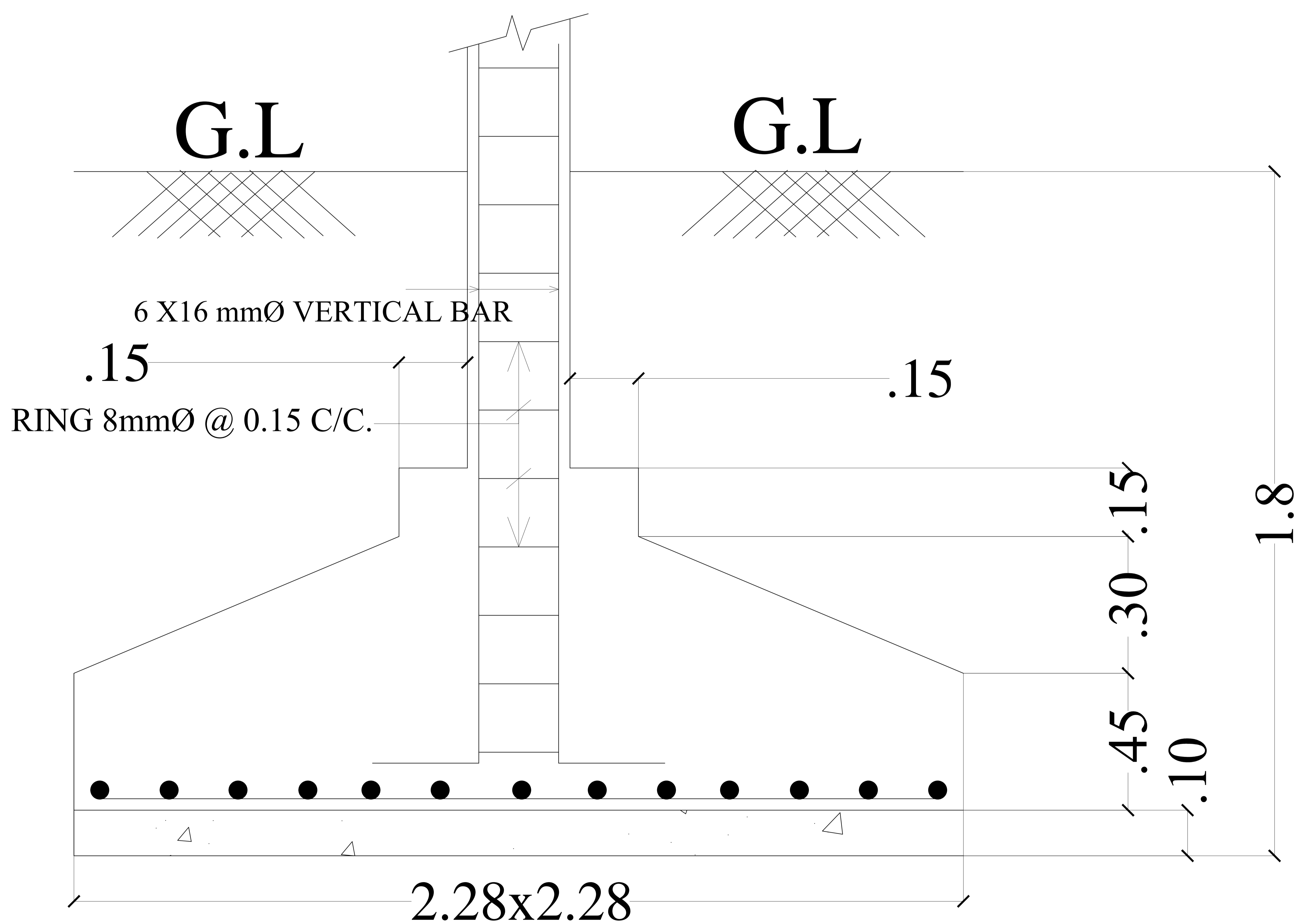
SECTION OF FOOTING
