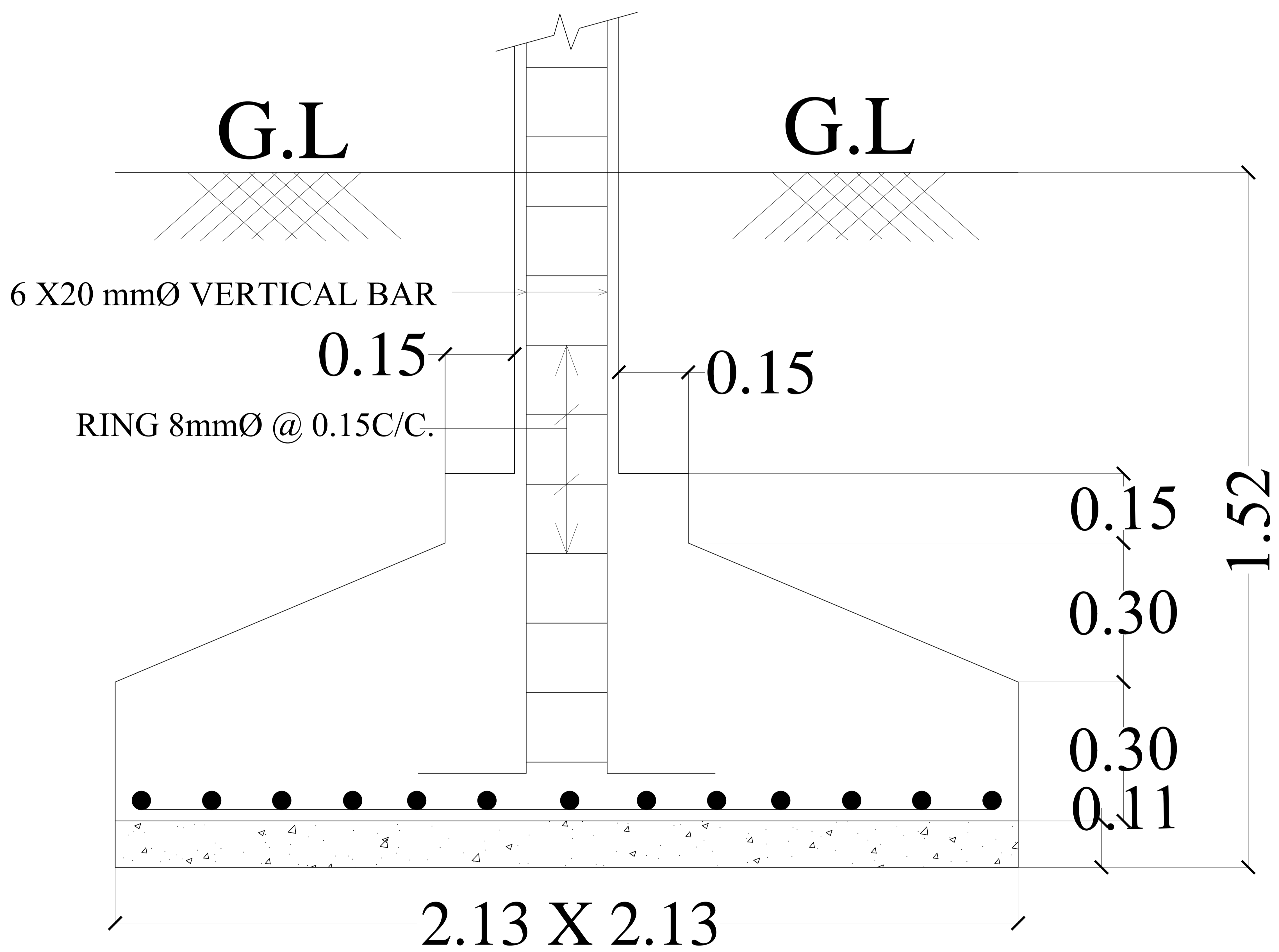
SECTION OF FOOTING
