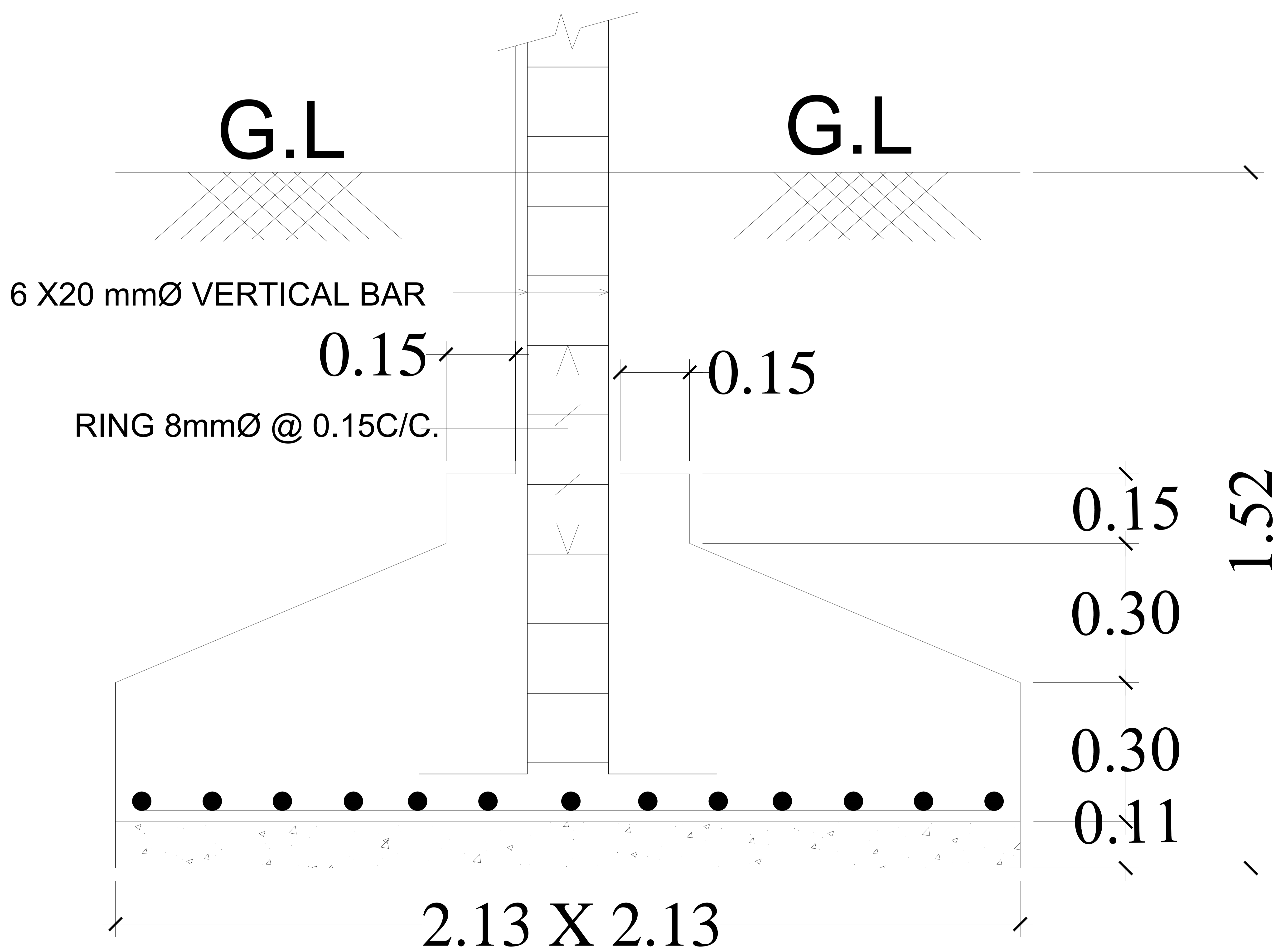
SECTION OF FOOTING
