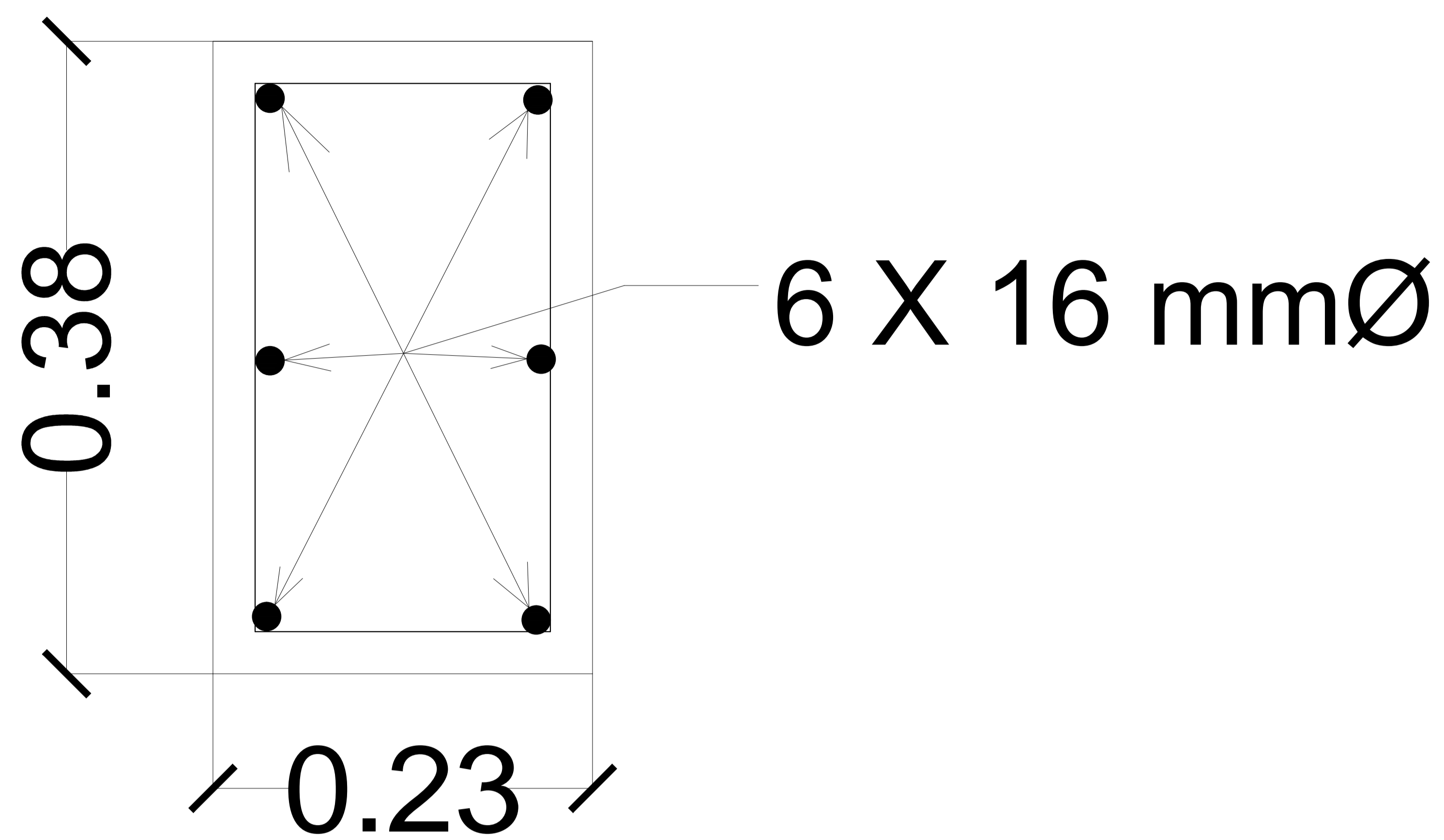
SECTION OF COLUMN.
