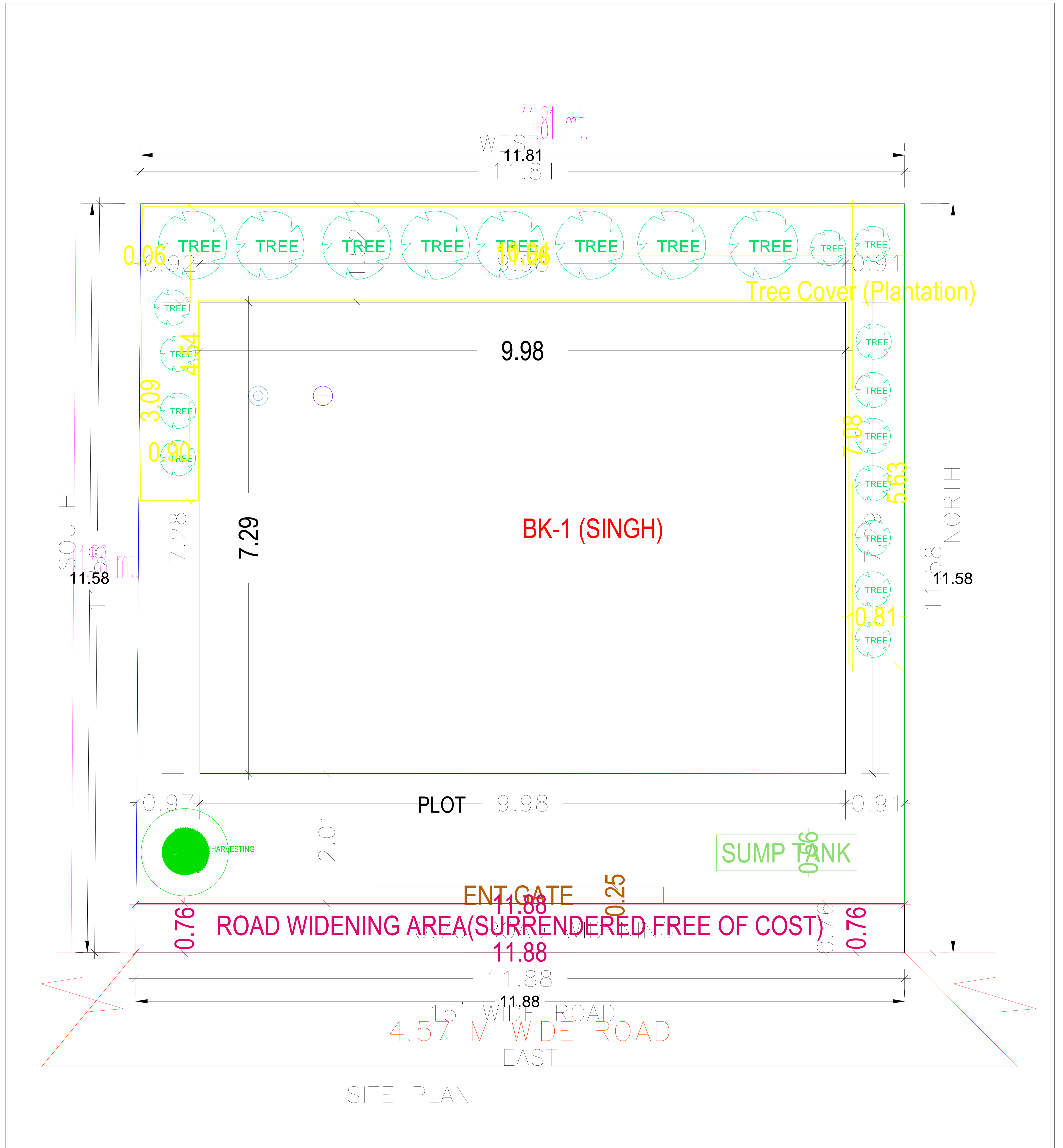
SITE PLAN
