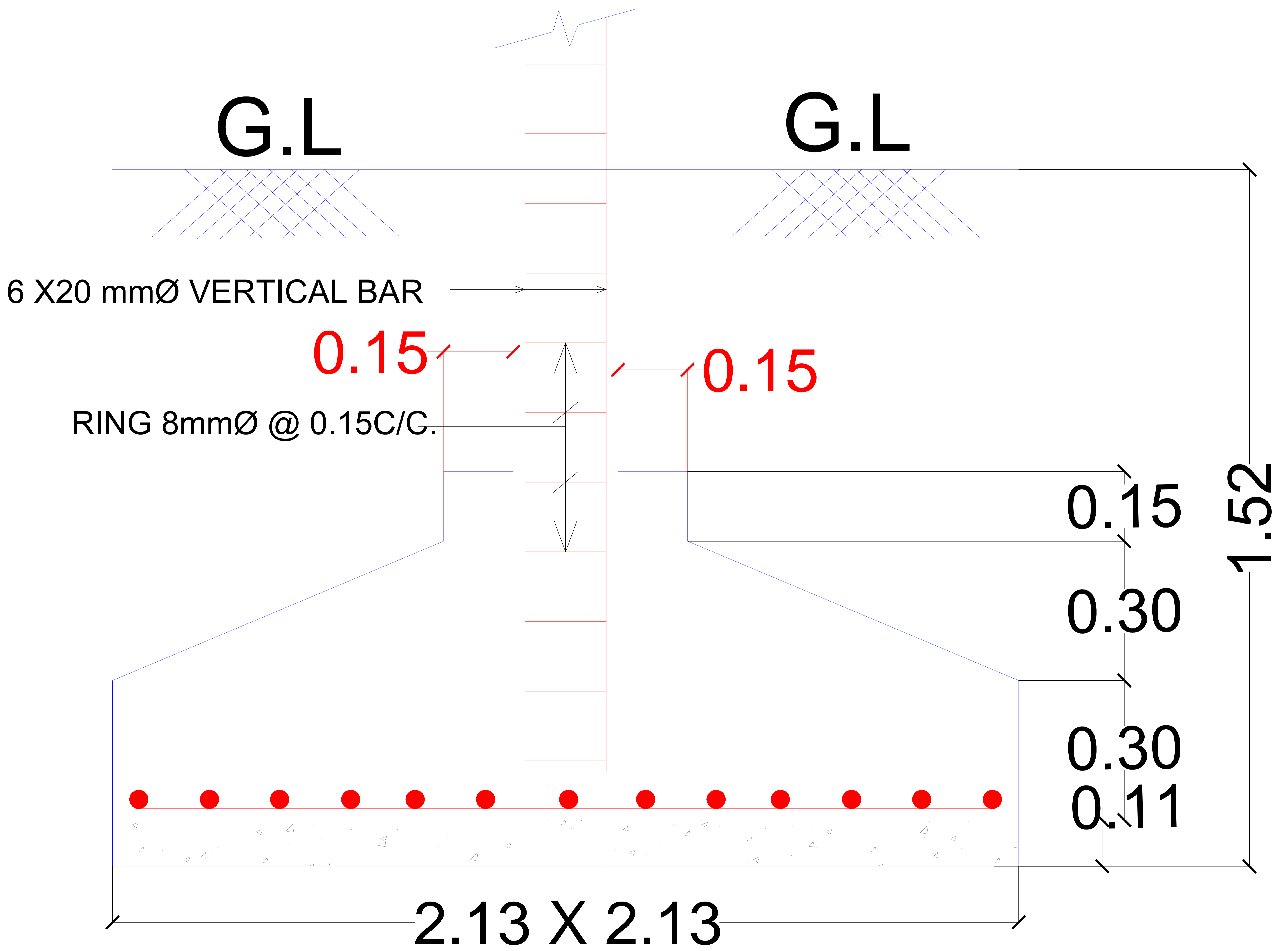
SECTION OF FOOTING
