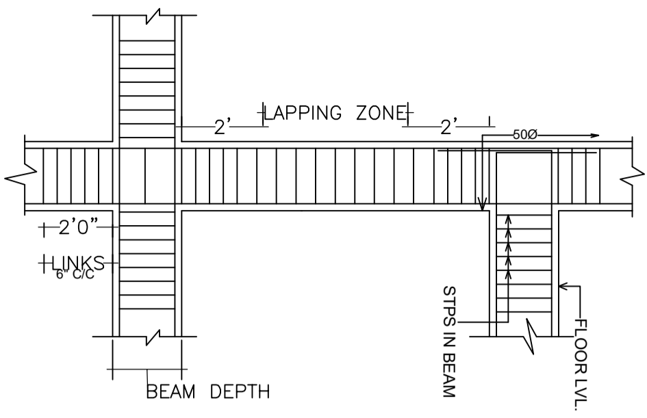
TYPICAL CROSS SECTION OF COLUMN BEAM
