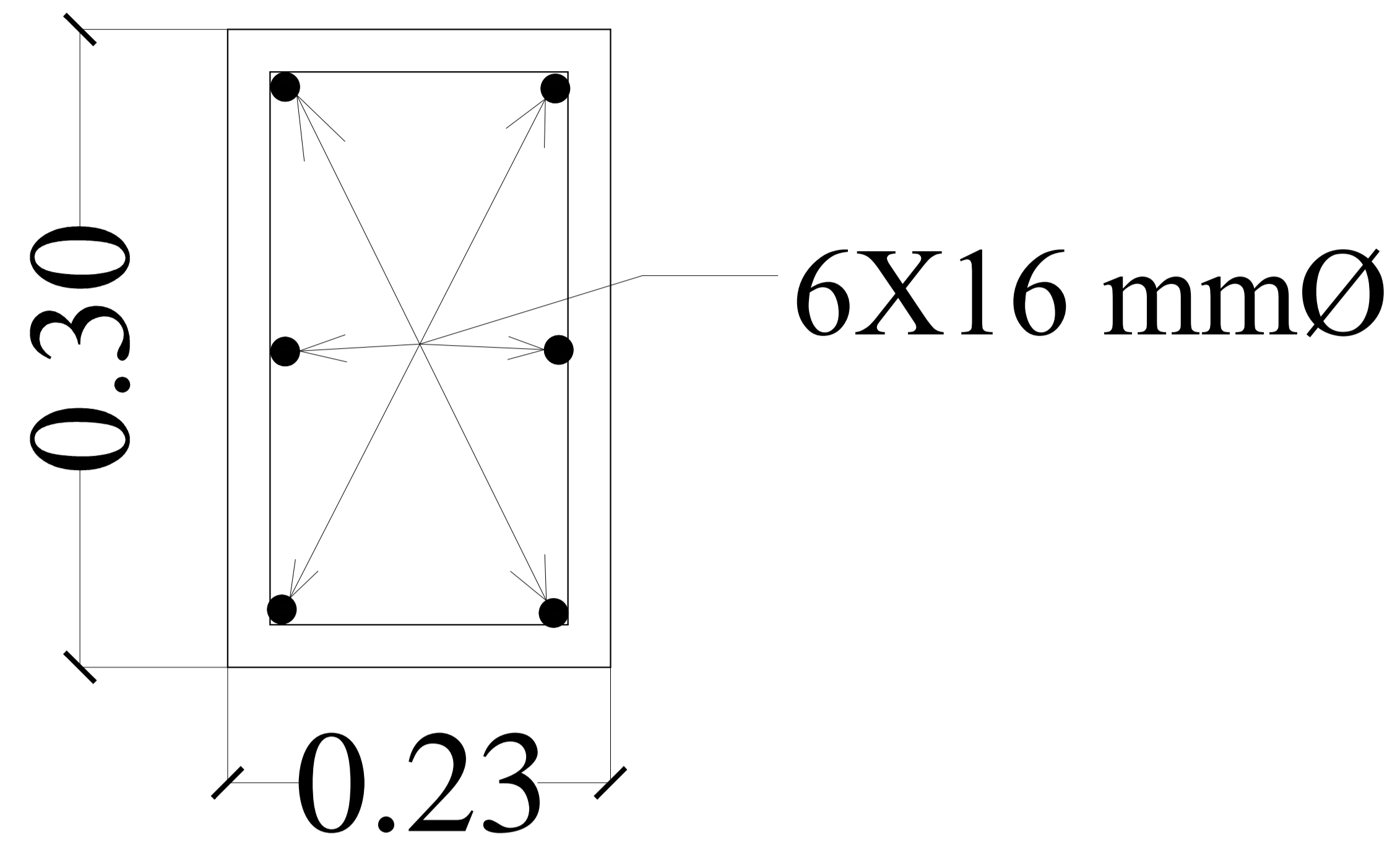
SECTION OF COLUMN
