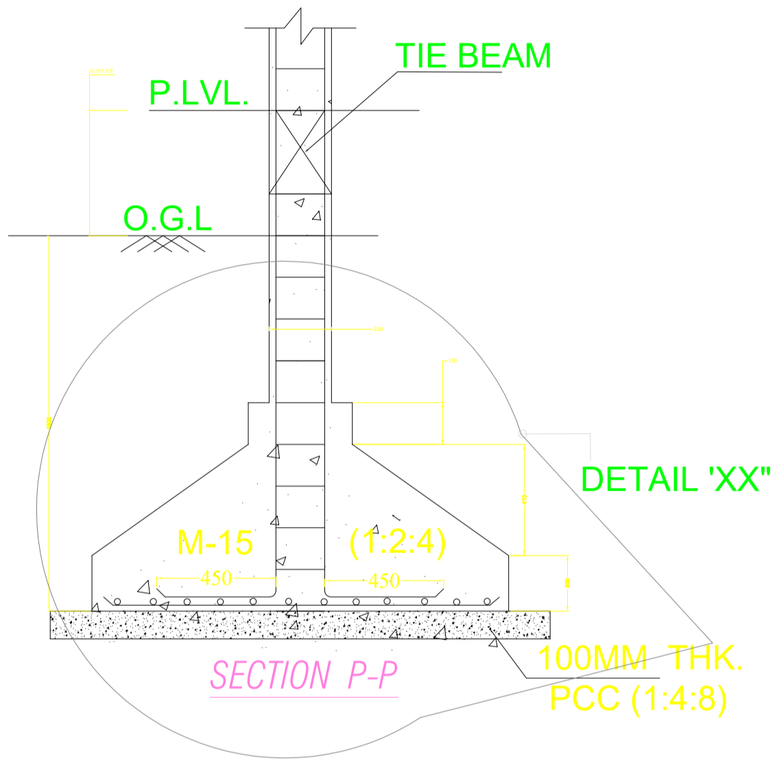
C/S OF COL.
