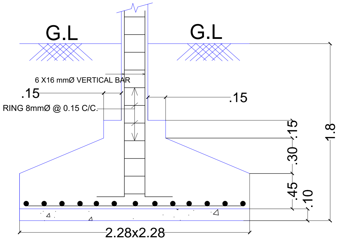
SECTION OF FOOTING
