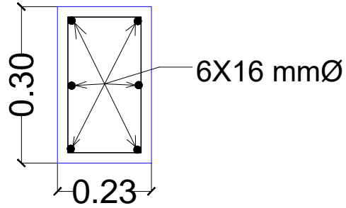
SECTION OF COLUMN
