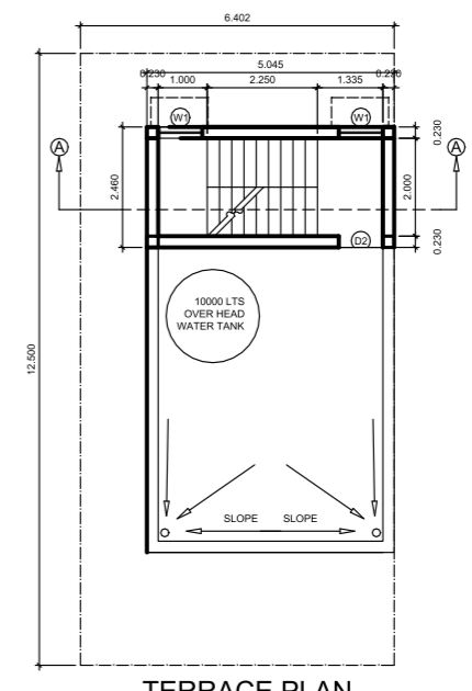
TERRACE PLAN SCALE- 1:75
