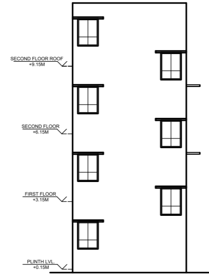
REAR ELEVATION SCALE- 1:75
