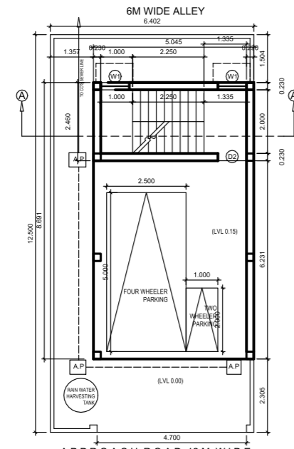
GROUND FLOOR PLAN SCALE- 1:75
