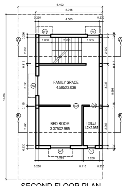
SECOND FLOOR PLAN SCALE- 1:75
