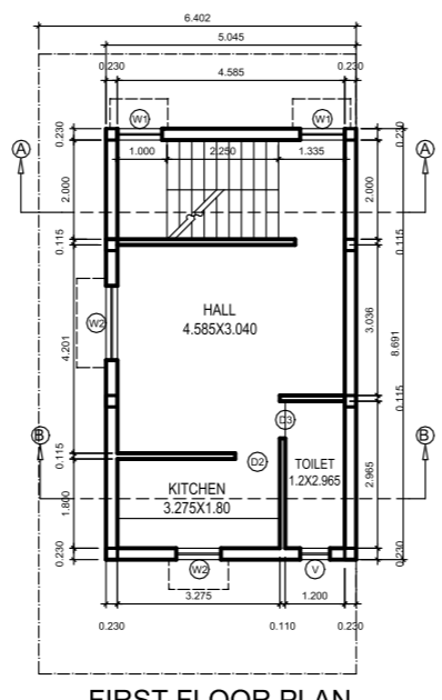
FIRST FLOOR PLAN SCALE- 1:75
