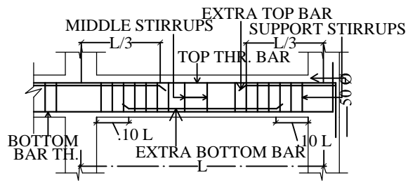
SECTION OF TYPICAL FLOOR BEAM
