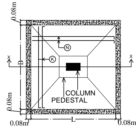
PLAN OF ISOLATED FOOTING
