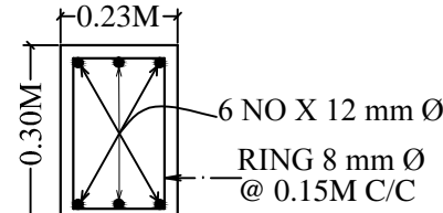
C.S. OF TIE BEAM SIZE - 0.23M X 0.30M
