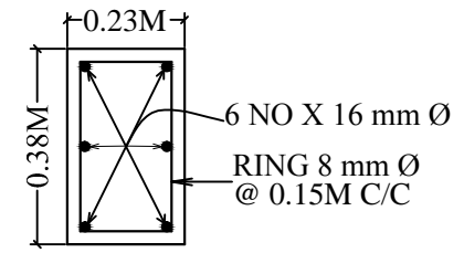
C.S. OF COLUMN SIZE - 0.23M X 0.38M
