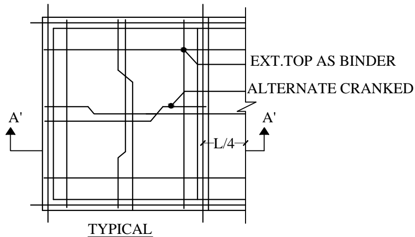
THICKNESS OF SLAB = 0.11m
