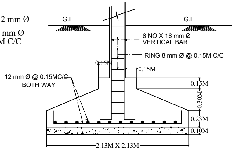
SECTION OF FOOTING SIZE - 2.13M X 2.13M
