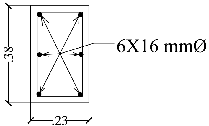
SECTION OF COLUMN. - C1
