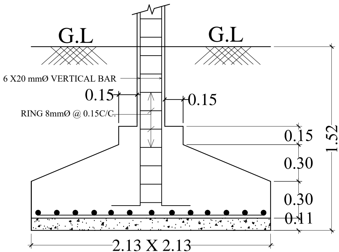
SECTION OF FOOTING
