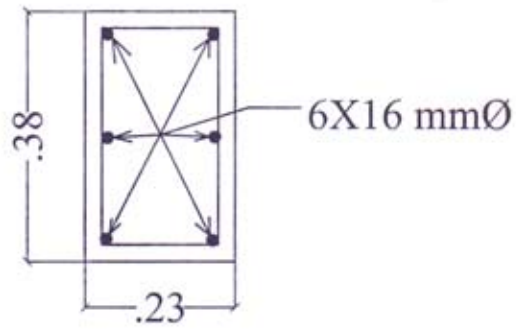
SECTION OF COLUMN. - C1
