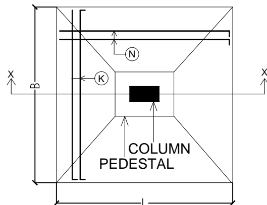
PLAN OF ISOLATED FOOTING
