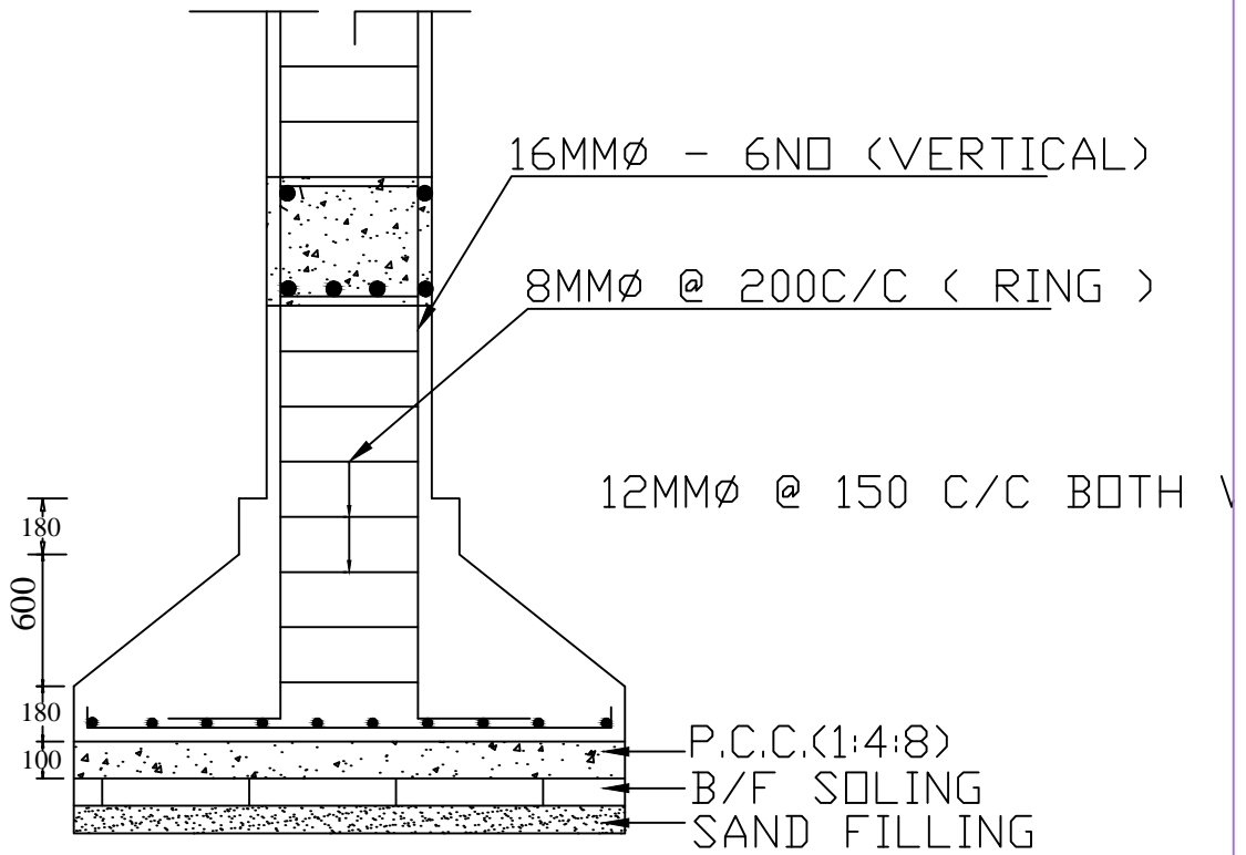
SECTION OF FOUNDATION
