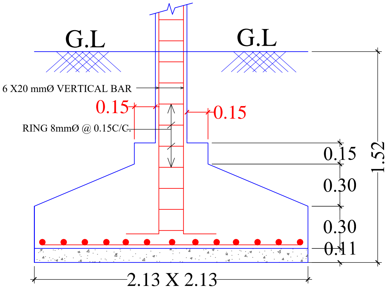
SECTION OF FOOTING
