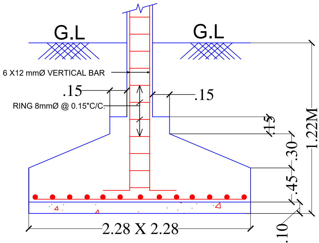
SECTION OF FOOTING
