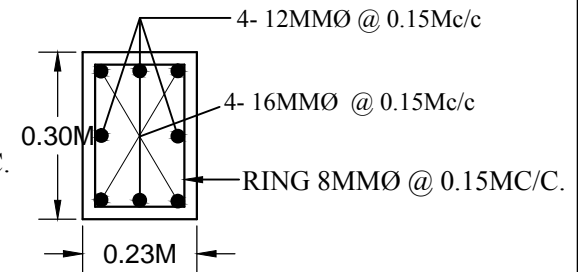
SECTION OF COLUMN
