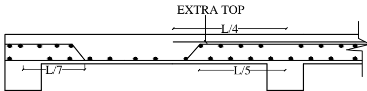
SECTION OF SLAB AT A-A'
