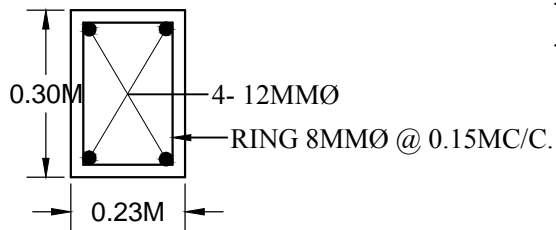
SECTION OF TIE BEAM
