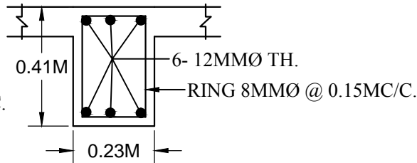
SECTION OF ROOF BEAM
