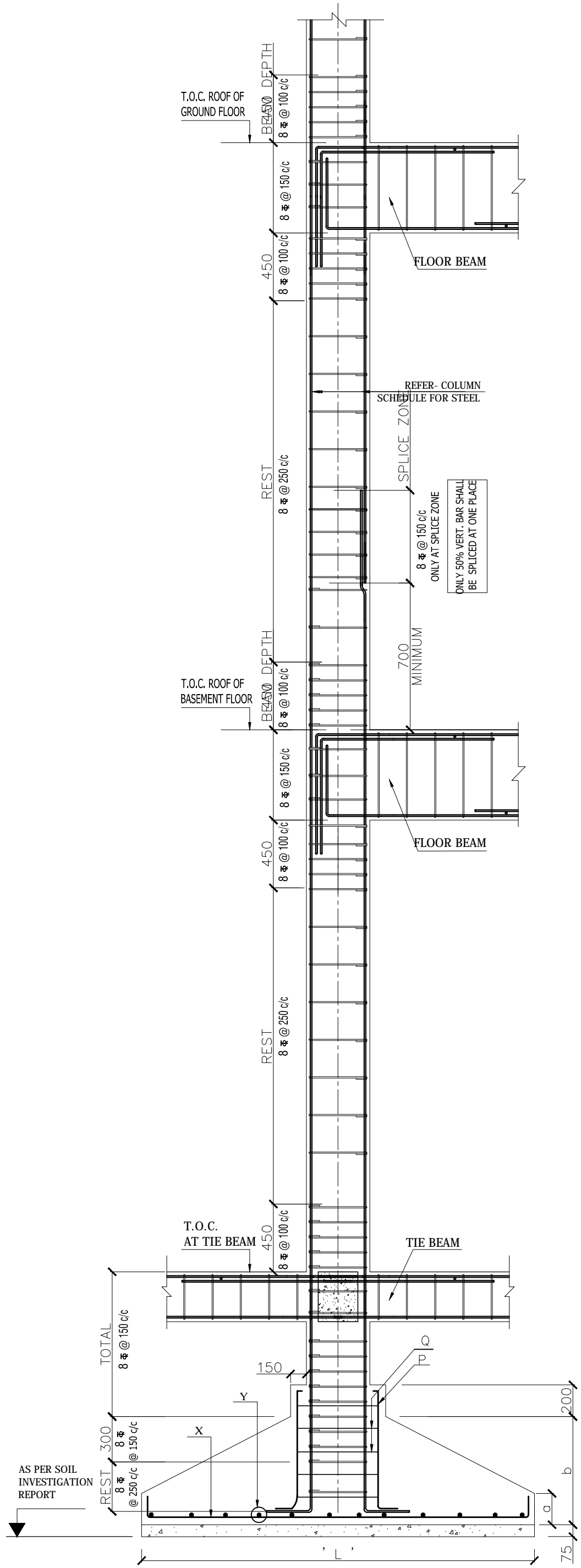
TYPICAL SECTION - COLUMN WITH FOUNDATION
