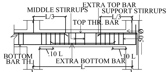
SECTION OF TYPICAL FLOOR BEAM
