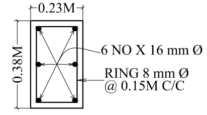
C.S. OF COLUMN . SIZE - 0.23M X 0.38M
