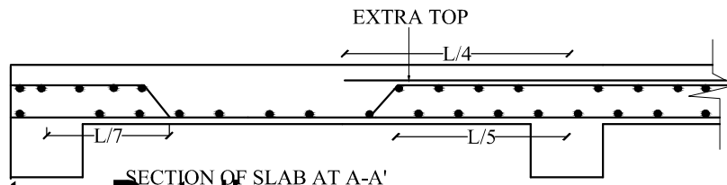
SECTION OF SLAB AT A-A'
