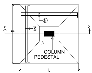
PLAN OF ISOLATED FOOTING
